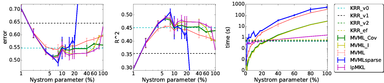
FIGURE 2 – Regression on Sarcos1-dataset. Left : normalized mean squared errors (the lower the better), middle : R^2 -score (the higher the better), right : running times ; as functions of Nyström approximation level (note the logarithmic scales). The results for KRR are calculated without approximation and are shown as horizontal dashed lines. Results for view 2 and early fusion are worse than others and outside of the scope of the two plots.
