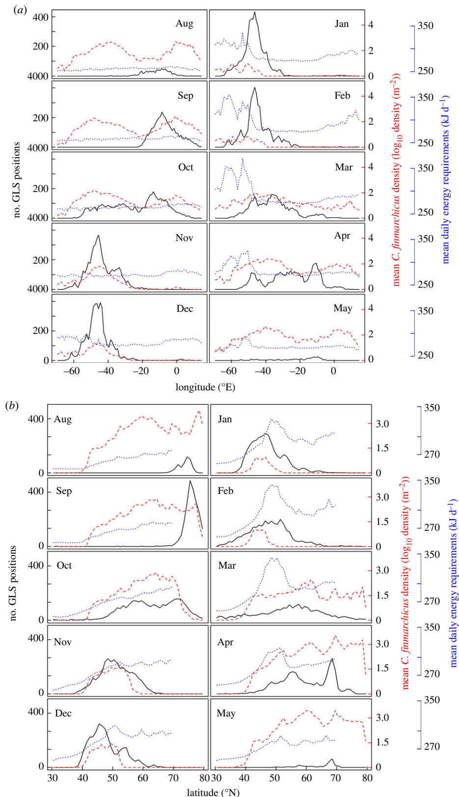
Figure 2. Number of little auk GLS positions (black), mean Calanus finmarchicus density in log 10 density m -2 (red, dashed line) and little auk mean daily energy requirements in kJ d -1 (blue, dotted line) per longitude (a) and latitude (b) and per month. The numbers of positions are low in August and May because most of the birds are already above the polar circle and permanent daylight does not allow positioning using GLS recorders. Similarly, bird position is not indicated during the summer (June and July), but their position was known as they were breeding at our study site in East Greenland.
