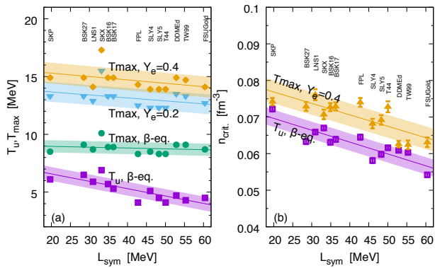
FIG. 5. (a) dissolution temperature T_u and maximal temperatures T_{max} at \beta -equilibrium, compared to T_{max} at fixed x_e=0.2 and 0.4 for the set of EOS compatible with chiral EFT EOS in neutron matter. (b) Highest density reached by the pasta phase for beta equilibrium or at fixed Y_e . These predictions are shown versus L_{sym} .
