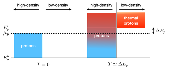
FIG. 3. This schematic shows the occupied proton energy levels in the low and high density phases that coexist in the heterogeneous phase. The T = 0 situation is shown on the left and finite temperature where a significant thermal population exists in the low density phase is shown on the right. See text for additional details.
