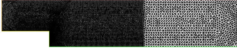
FIGURE 2. Triangular mesh of the channel - 16 425 triangles and 8 846 vertices.
