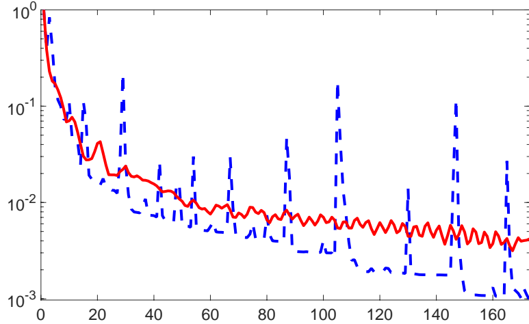
FIGURE 5. Evolution of \|\mathbf{g}^k\|_{\mathcal{A}}/\|\mathbf{g}^0\|_{\mathcal{A}} for the CG method (red line) and for the BB method (blue dashed line) w.r.t. iterate k - \nu = 1/50 .
