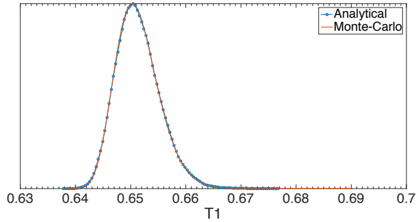
Figure 18: Probability density function \pi(T_1|\sigma = 0.35) at t = 0.034 s
