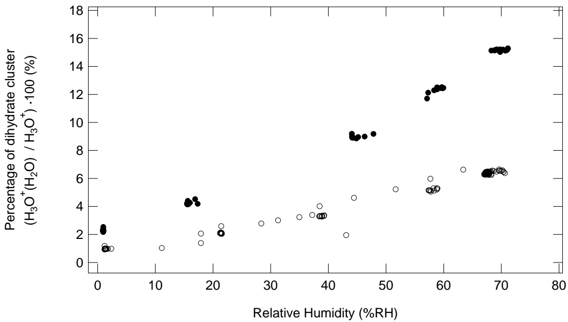
Figure 4: Plot of the fraction of the dihydrate cluster in the drift tube versus relative humidity. Experimental conditions: T = 298\text{K} , E/N = 140\text{Td} (open circles \circ ), E/N = 127\text{Td} (closed circles \bullet ). The percentage data of dihydrate clusters were calculated using the following equation: \frac{[\text{H}_2\text{O}-\text{H}_3^{18}\text{O}^+] \times 250}{[\text{H}_3^{18}\text{O}^+] \times 500} \times 100
