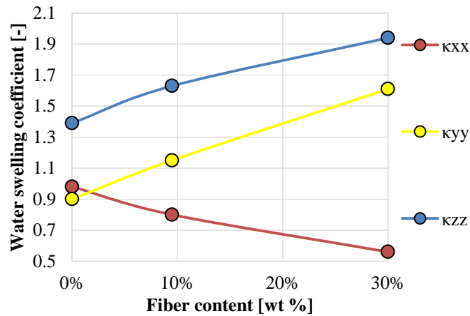
Figure 6 – Water swelling coefficients depending on each space direction for ISO IBA geometry (c.f. Figure 1) of PLA and flax/PLA composites
