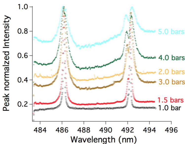
Figure 8. Superposition of six experimental spectra of the He I 492 nm ( right peak ) and H-β 486.2 nm ( left peak ) lines measured at room temperature for pressures in the range 1–5 bars. Black: 1 bar, red: 1.5 bars, light brown: 2 bars, dark brown: 3 bars, green: 4 bars, and blue: 5 bars.
