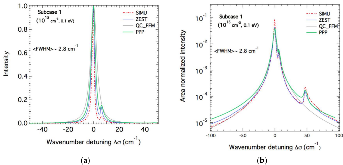
Figure 1. Theoretical Stark profiles of the He I 492 nm line calculated for helium plasma with an electron density of 10^{15} \text{ cm}^{-3} and a temperature of 0.1 eV for both plasma He + ions and electrons corresponding to subcase 1. The profiles are centered at 492 nm and expressed as wavenumbers using \text{cm}^{-1} units. (a) Linear scale. (b) The profiles are the same but they are area normalized and plotted using a semi-logarithmic scale to highlight the differences between the different calculations. In both (a,b), the average FWHM is shown. Red dot-dashed line: SimU, solid blue: ZEST, solid green: PPP, solid grey: QC_FFM.
