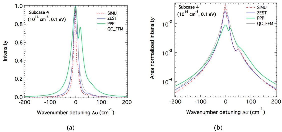
Figure 4. Theoretical Stark profiles of the He I 492 nm line calculated for a helium plasma with an electron density of 10^{16} \text{ cm}^{-3} and a temperature of 0.1 eV for both plasma He + ions and electrons. The profiles are centered at 492 nm and expressed as wavenumbers in \text{cm}^{-1} units. Blue: ZEST, green: PPP, grey: QC_FFM, red dot-dashed: SimU. (a) Linear scale. (b) Same profiles but area normalized and plotted using a semi-logarithmic scale.
