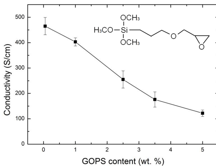
Figure 1. Electrical conductivity of PEDOT: PSS films cast from dispersions with GOPS concentration of 0.05, 1, 2.5, 3.5, and 5 wt%. Error bars result from error propagation taking into account 9 measurements, and the standard deviation in film thickness determination. The chemical structure of GOPS is given in the inset to the figure.
