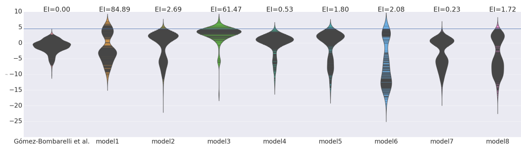
Figure 2: Violin plots showing the distributions of J(\text{eq.3}) of the molecules generated by the top 8 of our models and the ones generated by the model proposed in (Gómez-Bombarelli et al., 2016a). The blue horizontal line corresponds to the highest value of J in the training data, J^*(D) = 4.52 . We report the expected improvement EI * 10^3(\text{eq.2}) of each model. We can see that our models exhibit more diversity than the baseline (Gómez-Bombarelli et al., 2016a), this allows them to find molecules with better scores.
