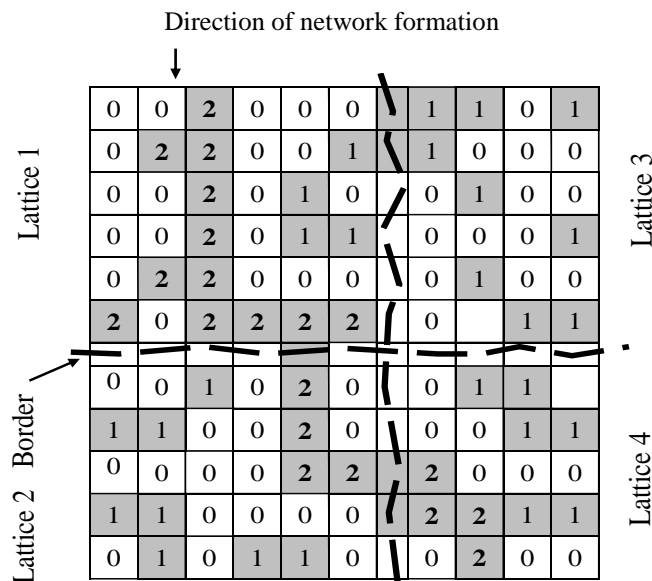
Legend: 0 – no percolation; 1 – network (internal cluster); 2 – network (cross-border percolation cluster)
