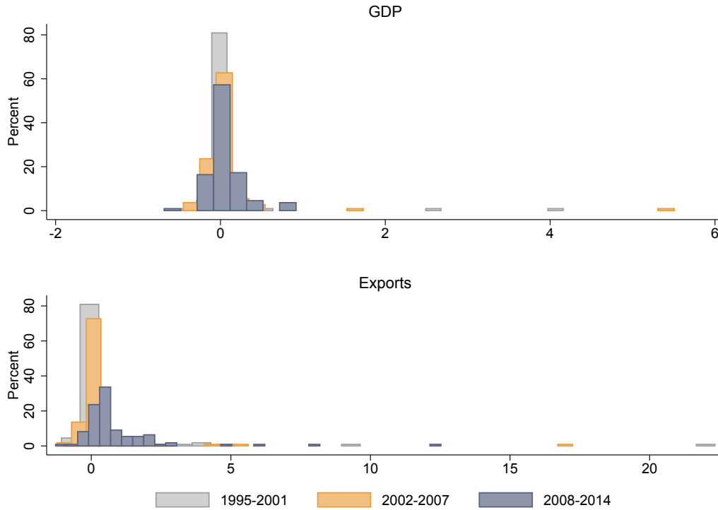
Figure 10: Distribution of GE Effects: False Positives CHN
