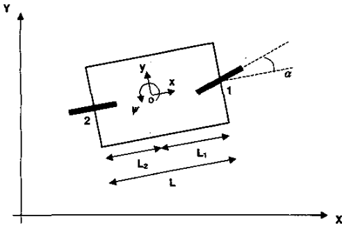
Figure 1: Bicycle model.
