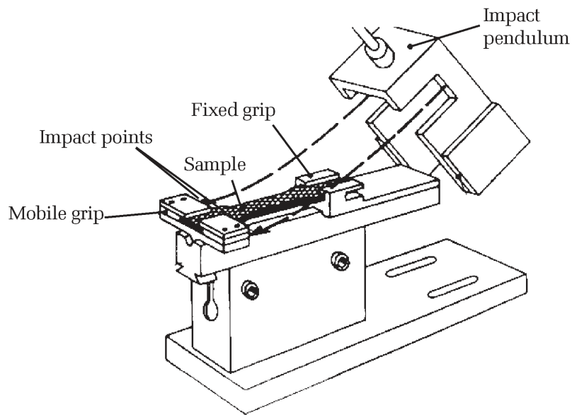
Figure 3. Principle of the pendulum tensile-impact machine
