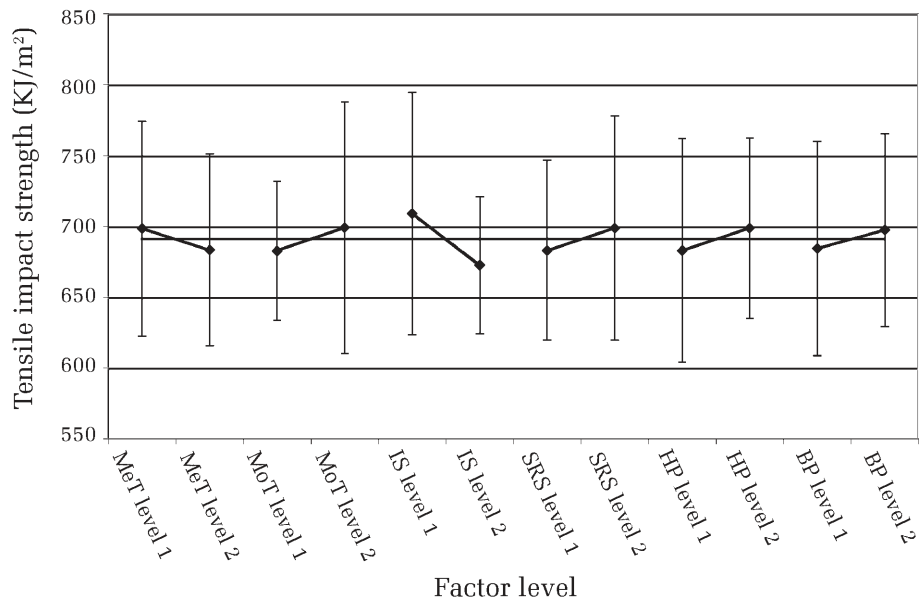
Figure 9. Effects of processing parameters on the longitudinal tensile-impact strength (standard deviations represents data scattering when the considered factor is set up at its low (1) or high (2) level in the Taguchi DOE)
