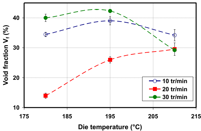
Fig. 4. Evolution of the void fraction in the foams of PLA 7000D ® as a function of the die temperature (180 °C, 195 °C and 210 °C) and at different screw speeds (10 rpm, 20 rpm and 30 rpm) – 2 wt% CFA – temperature A profile – slow cooling in air.
