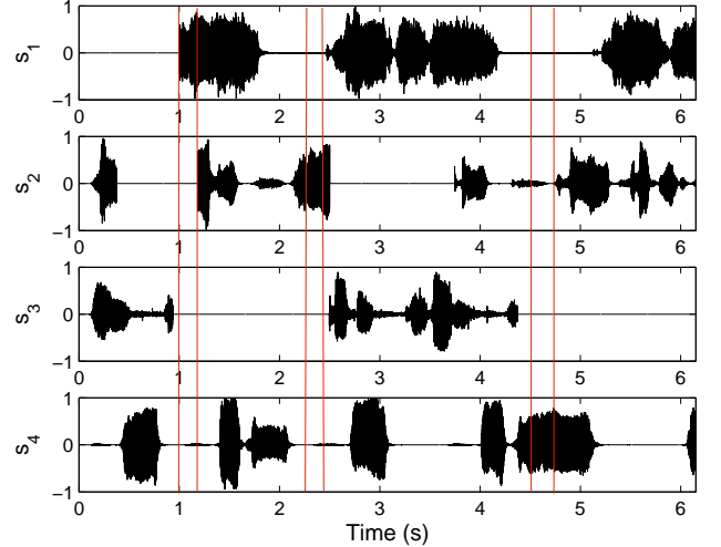
Fig. 2. Time representation of 4 audio sources: this representation illustrates the audio signal sparsity (i.e. there exists time intervals where only one source is present).
