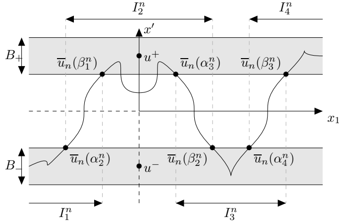
Figure 1: Possible trajectory for \bar{u}_n and the corresponding I_k^n
