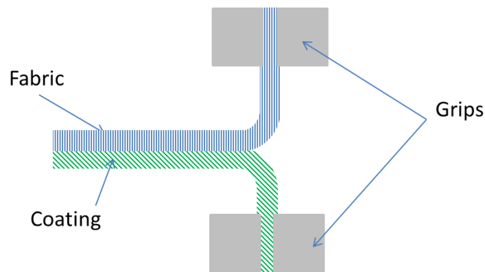
Figure 4: Scheme of the peel strength test according to standard NF EN ISO 2411
