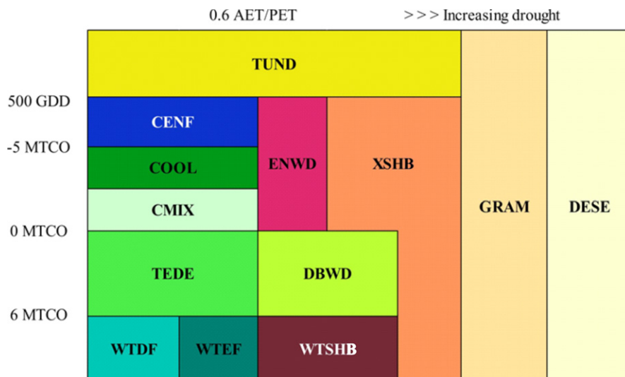
FIGURE 2 Conceptual model of the distribution of the 13 biomes recognized in the Eastern Mediterranean–Black Sea–Caspian biomes in climate space. MTCO: mean temperature of the coldest month, GDD: growing degree days, AET/PET: actual evapotranspiration/potential evapotranspiration. The biome codes are TUND: tundra, DESE: desert, GRAM: graminoids with forbs, XSHB: xeric shrubland, WTSHB: warm-temperate evergreen sclerophyll broadleaf shrubland, CENF: cold evergreen needleleaf forest, COOL: cool evergreen needleleaf forest, WTDF: warm-temperate deciduous malacophyll broadleaf forest, TEDE: temperate deciduous malacophyll broadleaf forest, CMIX: cool mixed evergreen needleleaf and deciduous broadleaf forest, WTEF: warm-temperate evergreen needleleaf and sclerophyll broadleaf forest, ENWD: evergreen needleleaf woodland, and DBWD: deciduous broadleaf woodland
