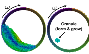
Granular material flow & granule growth in the cascading regime
