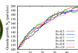
Exponential increase of granule for different Froude numbers.
