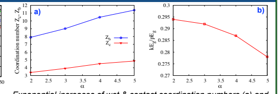
Exponential increases of wet & contact coordination numbers (a) and decrease of kinetic energy normalized by potential energy of granule (b), as functions of size ratio \alpha .
