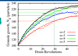
Exponential increase of granule for different size ratios
