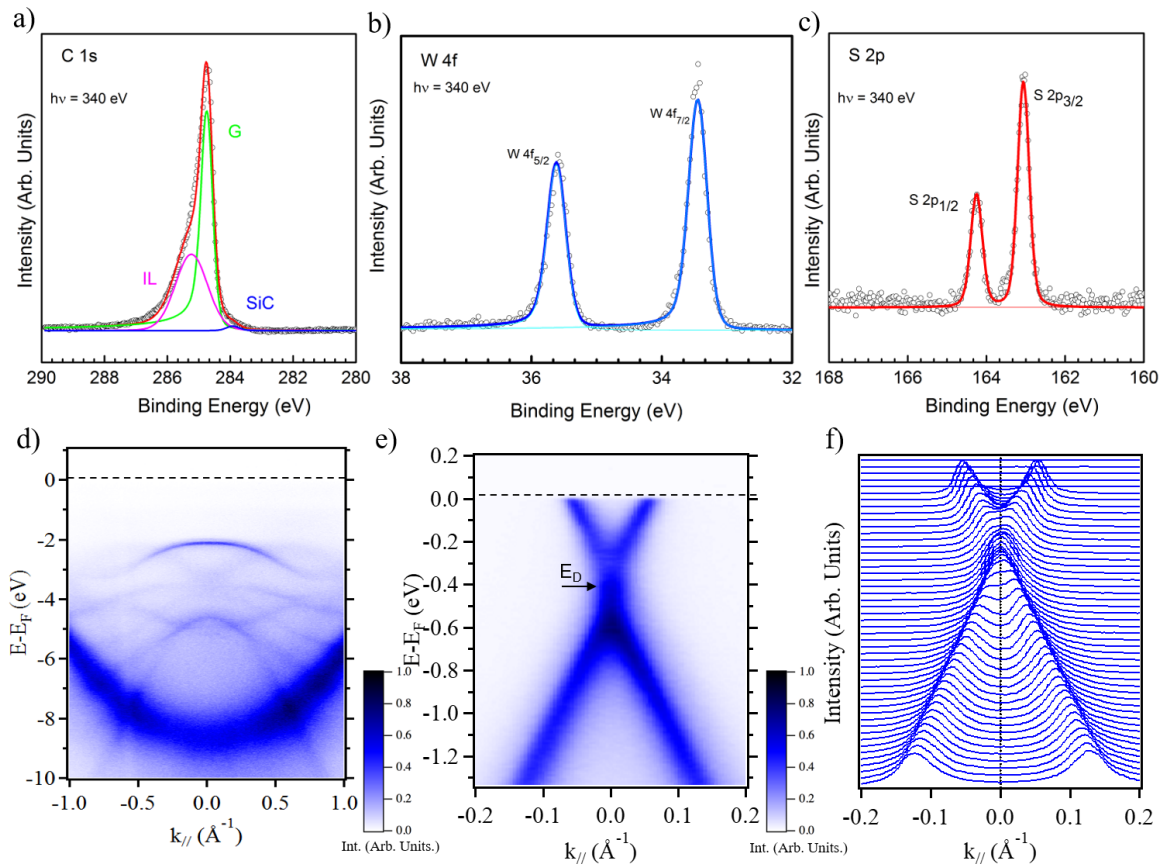
Figure 2: High resolution XPS and ARPES of WS 2 /graphene heterostructures: a) C-1s and b) W-4f , (c) S-2p core levels at h\nu = 340 eV. d) ARPES map of WS 2 /graphene heterostructure around the \Gamma point in the \Gamma K high symmetry direction of WS 2 Brillouin zone, e) Band structure of the graphene layer in the heterostructure at the \Gamma K high symmetry direction, f) corresponding momentum distribution curves (MDCs) of figure (e).
