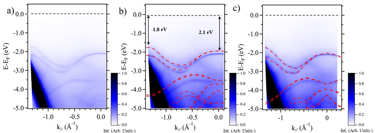
Figure 3: a) ARPES map of single layer WS 2 along the \Gamma K high symmetry directions, b) and c) Comparison between ARPES map and DFT calculations (PBE and HSE06 respectively).
