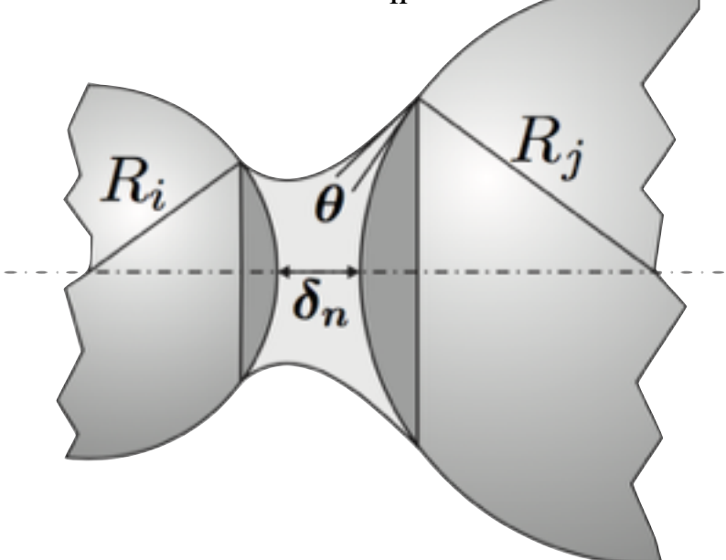
Diagram of capillary bridge
