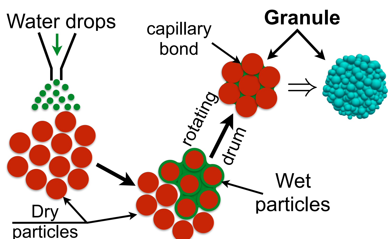
Mechanism of granule formation
