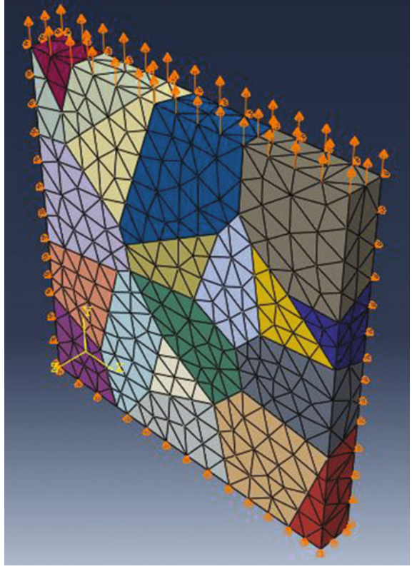
Fig. 2 Geometrical model and boundary condition of the polycrystal
