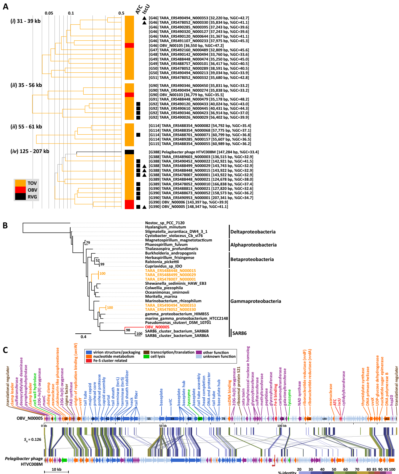
FIG 5 Genomes with Fe-S cluster assembly-related genes. (A) Four parts of the proteomic tree with genomes carrying Fe-S cluster assembly genes (i.e., ATC [■] and lscU [▲] genes). Branch lengths are logarithmically scaled as described for Fig. 3A. Genus-level gOTUs and genome identifiers (IDs), lengths, and percent G+C compositions are indicated. (B) Maximum likelihood tree of lscU genes. The tree contains protein sequences encoded in OBV_N00005 (red), five TOV-EVGs (orange), and 21 Proteobacteria and cyanobacterial genomes (black). The scale bar refers to the estimated number of amino acid substitutions per site. Numbers close to the nodes represent bootstrap percentages of >50%. The tree is rooted by the cyanobacterial Nostoc species sequence. (C) Genome map of OBV_N00005 and Pelagibacter phage HTVC008M. The HTVC008M sequence is circularly permuted at 97,000 bp and reversed. A red arrow indicates the original (Continued on next page)
