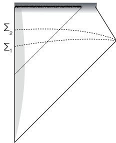
FIG. 1. The (lowest part) of the conformal diagram of a gravitational collapse. The clear grey region is the object, the dotted line is the horizon, the thick upper line is the singularity, the dark upper region is where quantum gravity effect may become relevant (this region play no role in this paper.) The two Cauchy surfaces used in the paper are the dashed lines.
