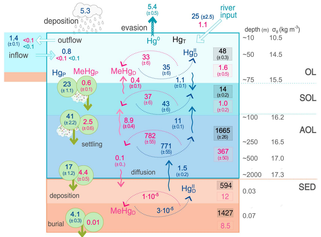
Figure 8. Budget for Hg species in the Black Sea. Modeled amount (kmol) and fluxes ( \text{kmol yr}^{-1} ) of \text{Hg}_T (black), \text{Hg}^{\text{II}} (blue) and \text{MeHg}_T (pink) species in water and sediment layers, given as mean \pm SE. \text{Hg}_T and \text{MeHg}_T reservoirs (black and pink squares) are given on the right side. \text{Hg}^0 (dark cyan) is produced upon net photoreduction in oxic waters and mostly evade to the atmosphere; its pool is a minor fraction of the \text{Hg}_T pool and is thus omitted here. Settling, deposition and burial of \text{Hg}_P and \text{MeHg}_P are represented by green circles and arrows. Fluffy arrows represent exchanges due to turbulent and molecular diffusion. Dashed arrows indicate methylation and demethylation. Thick arrows show exchanges at the model boundaries (atmospheric deposition and evasion, river load, and inflow-outflow to the Marmara Sea). On the right side depth and density scale are shown. OL = oxic layer; SOL = suboxic layer; AOL = anoxic layer.
