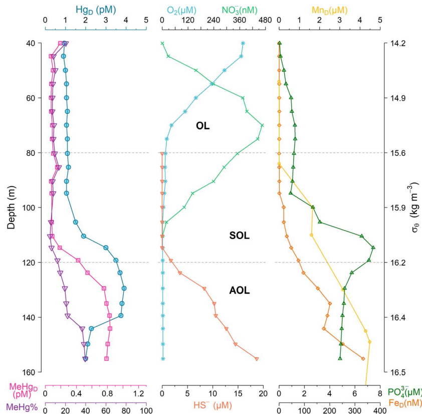
Figure 5. High-resolution profiles of dissolved Hg (Hg D ), and MeHg (MeHg D ), oxygen (O 2 ), hydrogen sulfide (HS - ), nitrates (NO 3 - ), phosphates (PO 4 3- ), manganese (Mn D ), and iron (Fe D ) at station 5 (Figure 1). OL = oxic layer; SOL = suboxic layer; AOL = anoxic layer.
