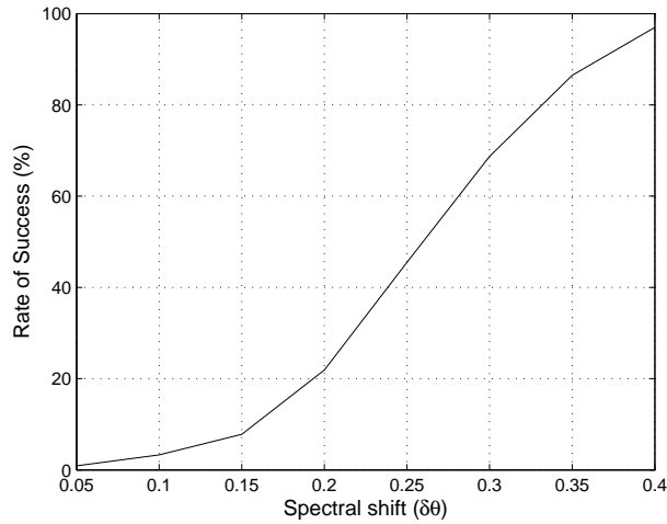
Fig. 12. Rate of success versus spectral shift \delta\theta for 2 autoregressive sources and 5 sensors and SNR = 25dB.
