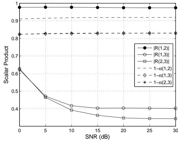
Fig. 13. Average values of the |\mathcal{R}(i, j)| and thresholds 1 - \alpha_{(i,j)} versus SNR for 3 sources and 3 sensors : 2 sources are complex white Gaussian processes and the third one is an autoregressive signal.
