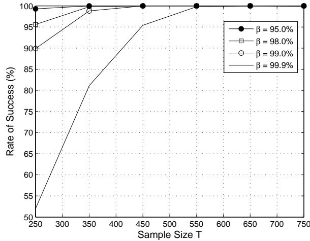
Fig. 10. Rate of success versus sample size T for 2 autoregressive sources and 2 sensors and SNR = 25dB: comparison of the performance of our algorithm for different confidence interval \beta .
