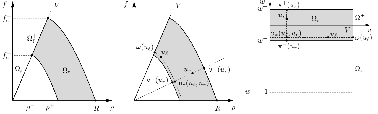
Figure 1: Notations.
