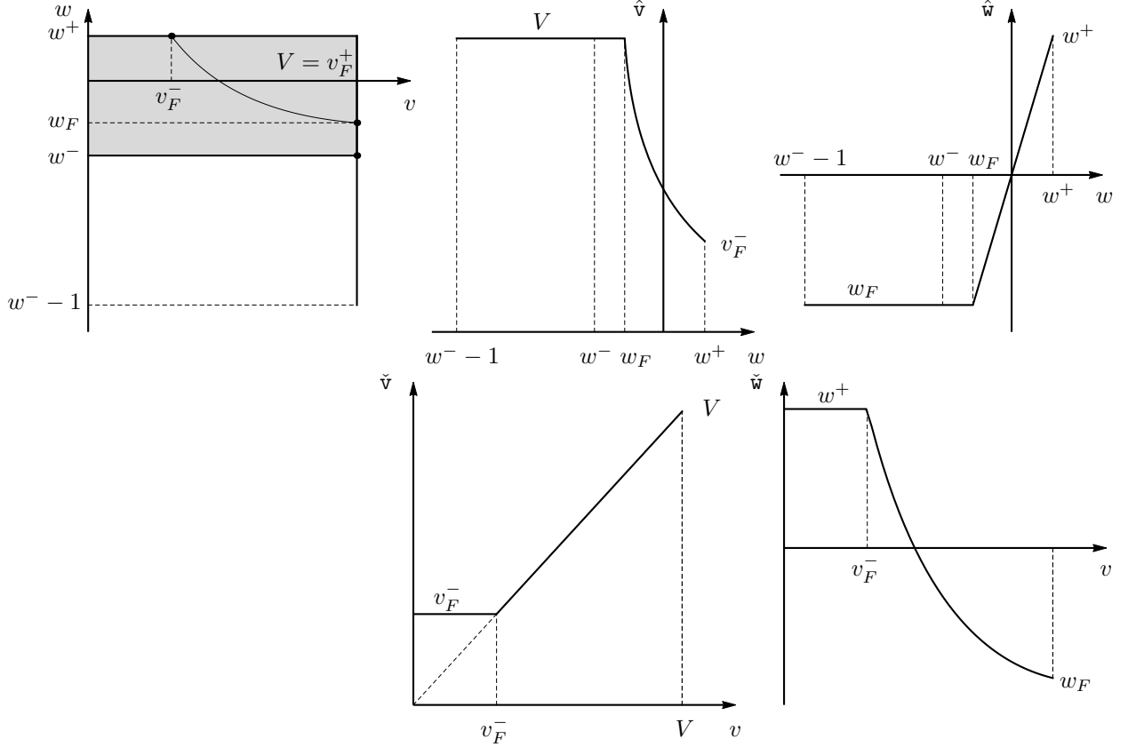
Figure 3: Geometrical meaning of \hat{u} and \check{u} defined in (11) in the case F \in (f_c^-, f_c^+) .
