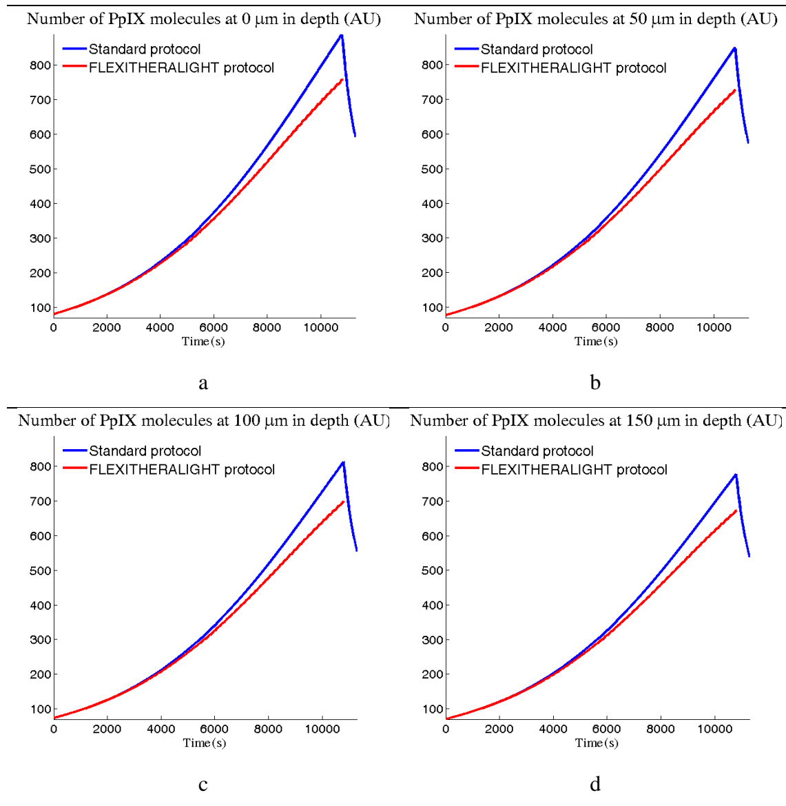
Figure 4: Evolution in time of the number of PpIX molecules when using the standard protocol (incubation time: three hours, irradiation type: continuous, light dose: 37 \text{ J/cm}^2 , fluence rate: 75 \text{ mW/cm}^2 , treatment duration: 493 s) (blue curves) and the FLEXITHERALIGHT one (incubation time: 30 minutes, irradiation type: fractionated with two minutes dark intervals every three minutes, light dose: 37 \text{ J/cm}^2 , fluence rate: 12.3 \text{ mW/cm}^2 , treatment duration: 9024 s) (red curves) at 0 (a), 50 (b), 100 (c) and 150 (d) \mu\text{m} in depth in AK.
