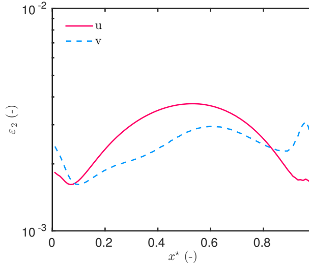
Figure 13. \ell_2 error for the two fields u(x, t) and v(x, t) .
