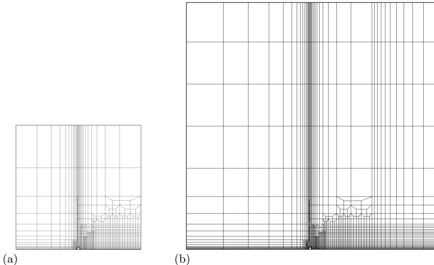
Figure 3: View of the cylinder mesh M1 : (x_{1,u}, x_{1,d}, y_1) = (-25, 25, 50) (left image) and M2 : (x_{2,u}, x_{2,d}, y_2) = (-50, 50, 100) (right image). The cylinder is placed in the middle of the x -axis, and near the wall at a gap ratio of G/d = 0.005 in order to avoid numerical singularities from arising. The flow is from left to right, and the resolution in the vicinity and downstream of the cylinder is increased in order to accurately capture the flow structures in the wake.
