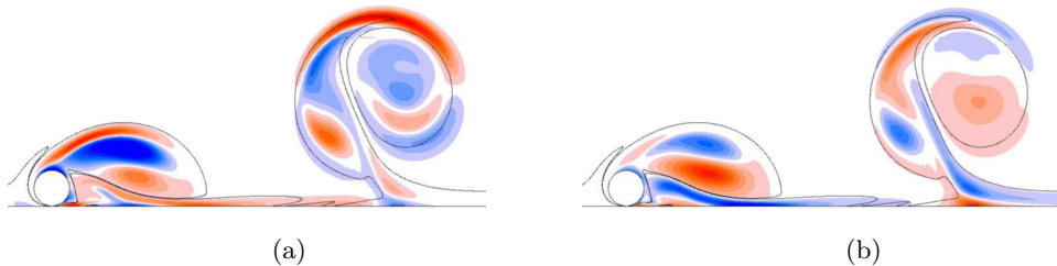
Figure 13: Visualisations of the streamwise perturbation vorticity for subharmonic mode (3) (left) and real mode (5) (right) at Re = 160 . These images depict streamwise perturbation vorticity coloured contours with base flow vorticity contour line at \pm 0.1d/U overlaid to highlight the locations of the vortices.
