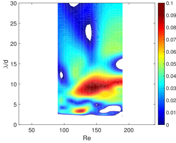
Figure 10: Contour map of the dominant growth rate \sigma as a function of the Reynolds number Re and the wavelength \lambda/d for the 2D periodic base flow.
