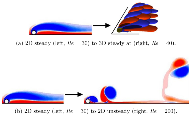
Figure 4: Visualisation of the initial flow transitions under consideration. The images showing 2D flow depict the spanwise vorticity field, whereas the 3D flow pattern is depicted using isosurfaces of streamwise vorticity. Red and blue represent positive and negative vorticity, respectively.
