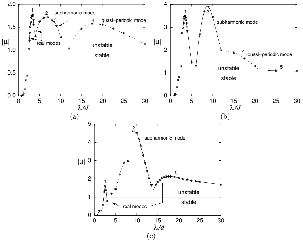
Figure 11: Floquet multiplier variation against spanwise wavelength for the dominant Floquet mode at each wavelength for Re = 100 (a), Re = 130 (b) and 160 (c).
