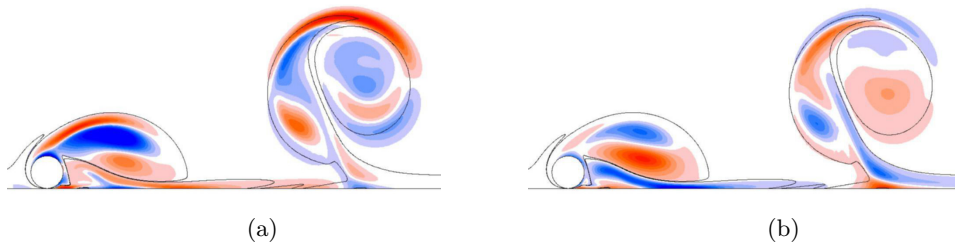
Figure 13: Visualisations of the streamwise perturbation vorticity for subharmonic mode (3) (left) and real mode (5) (right) at Re = 160 . These images depict streamwise perturbation vorticity coloured contours with base flow vorticity contour line at \pm 0.1d/U overlaid to highlight the locations of the vortices.
