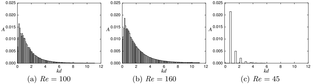
Figure 21: Time-mean amplitudes of saturated Fourier modes corresponding to the spanwise velocity component against dimensionless wavenumber kd for (a) Re = 100 and (b) Re = 160 . These are taken over the 100 time units after the asymptotic state is reached. The righthand image (c) shows the final mode amplitude distribution for Re = 45 , well below the transition to the periodic state.
