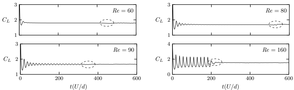
Figure 18: Temporal evolution of the lift coefficient from Re = 60 to 160 computed from the three-dimensional direct numerical simulations. The dashed ellipses show the instant at which the three-dimensional instability has grown sufficiently to alter the two-dimensional flow.
