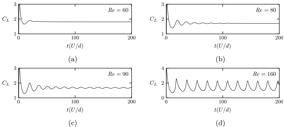
Figure 2: Time evolution (scaled by d/U ) of the lift coefficient from impulsive startup. (a) & (b) Evolution for Reynolds number below the transition to 2D shedding. (c) & (d) Evolution for Reynolds numbers beyond the transition to vortex shedding.
