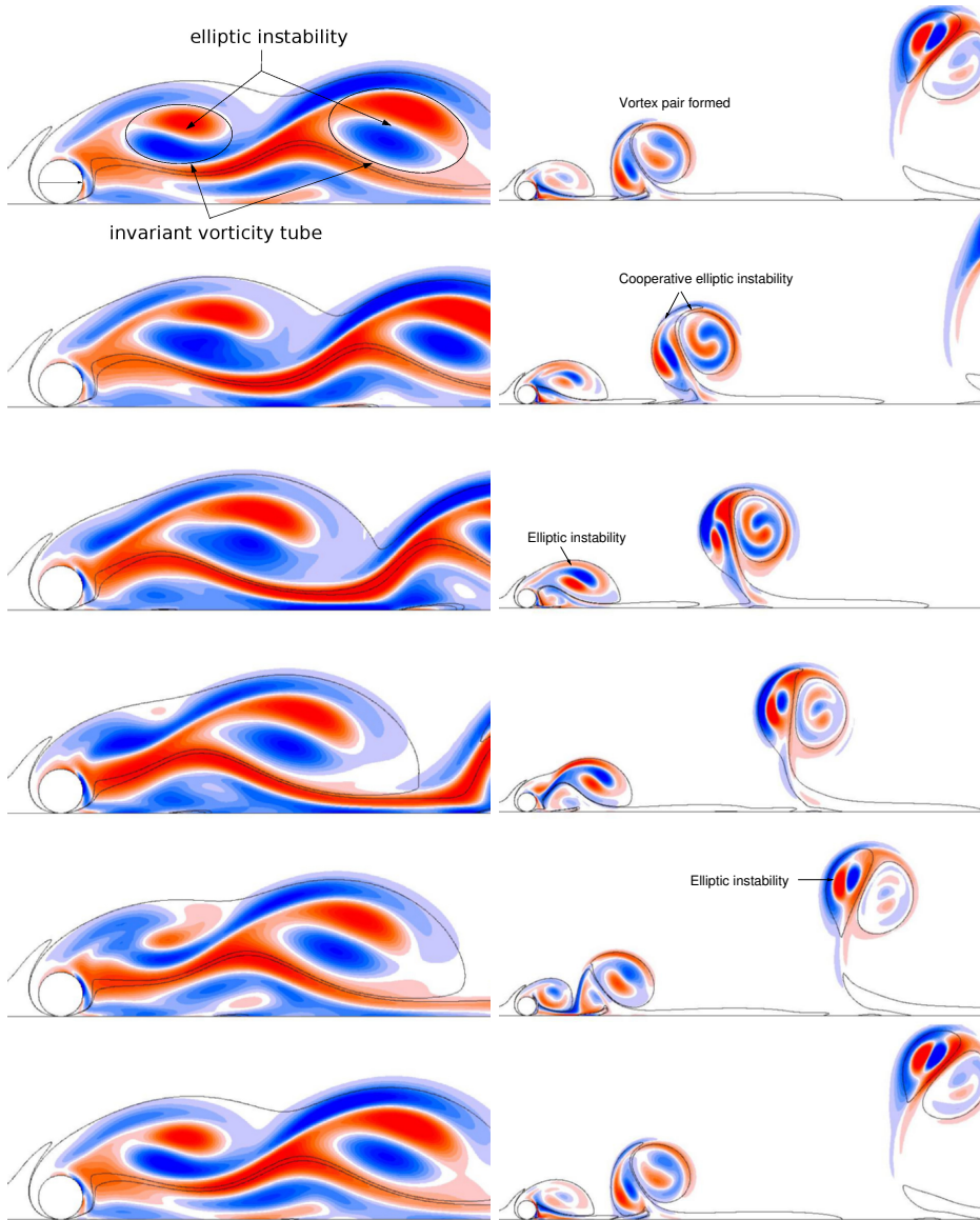
Figure 12: Evolution of the spanwise perturbation vorticity for the mode (1) of figure 11 at Re = 100 (left column) and Re = 160 (right column), overlaid with the base flow vorticity contours at \pm 0.1U/d . The images are 1/5 of a period apart. The spatial distribution of the instability fields show strong signs of elliptic instability of the vortex cores, as discussed in the text.
