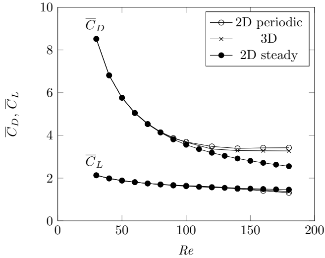
Figure 16: Comparison of time-averaged body force coefficients, drag \bar{C}_D and lift \bar{C}_L , between the two- and three-dimensional simulations for 30 \leq Re \leq 180 . Note that beyond Re_{c,2D} the 2D-steady predictions shown by the filled circles are based on flows calculated with the steady solver.
