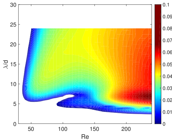
Figure 7: Contour map of the growth rate \sigma as a function of the Reynolds number Re and the wavelength \lambda/d for the 2D steady to 3D transition. For most of the domain, the dominant 3D mode is steady, except for a small (blue) region centred around Re = 120 and \lambda/d = 5 and extending to higher Reynolds numbers.
