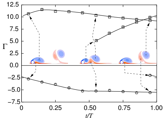
Figure 15: Evolution of the circulation \Gamma of the primary and secondary vortices over a shedding cycle as they form and advect downstream. Here, Re = 160 .
