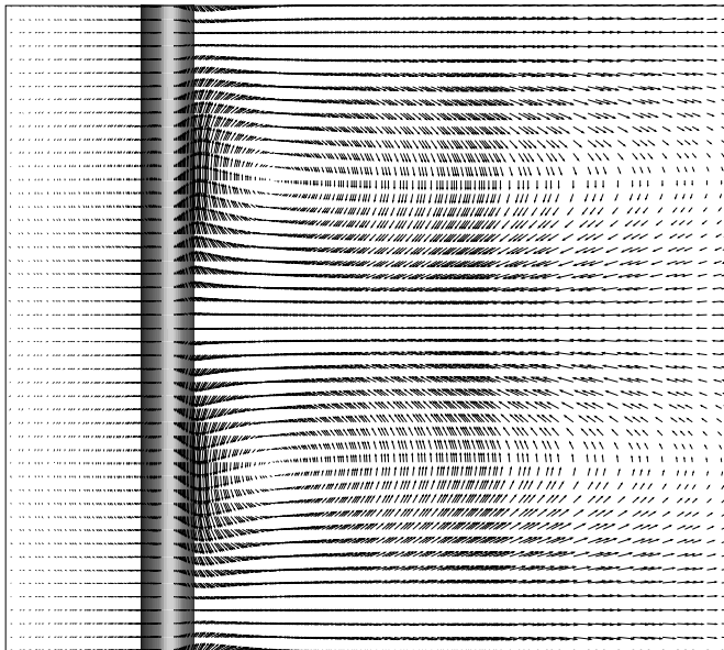
Figure 5: Top down view of the three-dimensional steady flow at Re = 60 and \lambda/d = 11 , depicted through the projected velocity field in the plane grazing the top of the cylinder.
