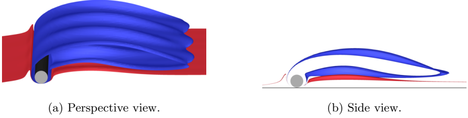
Figure 17: The fully developed wake state at Re = 50 visualised over a spanwise distance of three characteristic wavelengths. The wake state is depicted using an isosurface of the spanwise vorticity ( \omega_z = \pm 0.5 ).
