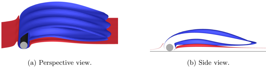
Figure 17: The fully developed wake state at Re = 50 visualised over a spanwise distance of three characteristic wavelengths. The wake state is depicted using an isosurface of the spanwise vorticity ( \omega_z = \pm 0.5 ).
