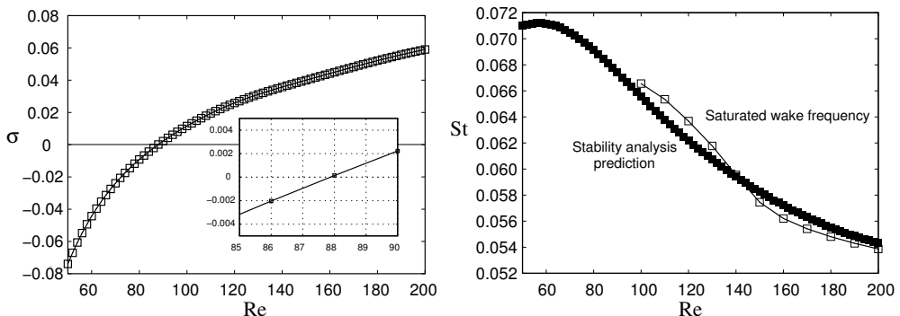
Figure 9: Left: Growth rate of most unstable mode from stability analysis applied to the rolling cylinder for 50 \leq Re \leq 200 . The lower inset shows the stability curve as it crosses the neutral stability line. Right: Predicted Strouhal number of the perturbation field compared to that of the saturated flow state.
