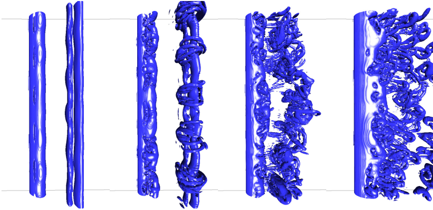
Figure 23: Stages in the evolution of the wake at Re = 160 as depicted by isosurfaces of Q = 0.01 . The first three images show the wake structure for three consecutive cycles just after the three-dimensionality is starting to modify the flow. The final image is a typical image after the flow has reached its asymptotic state.
