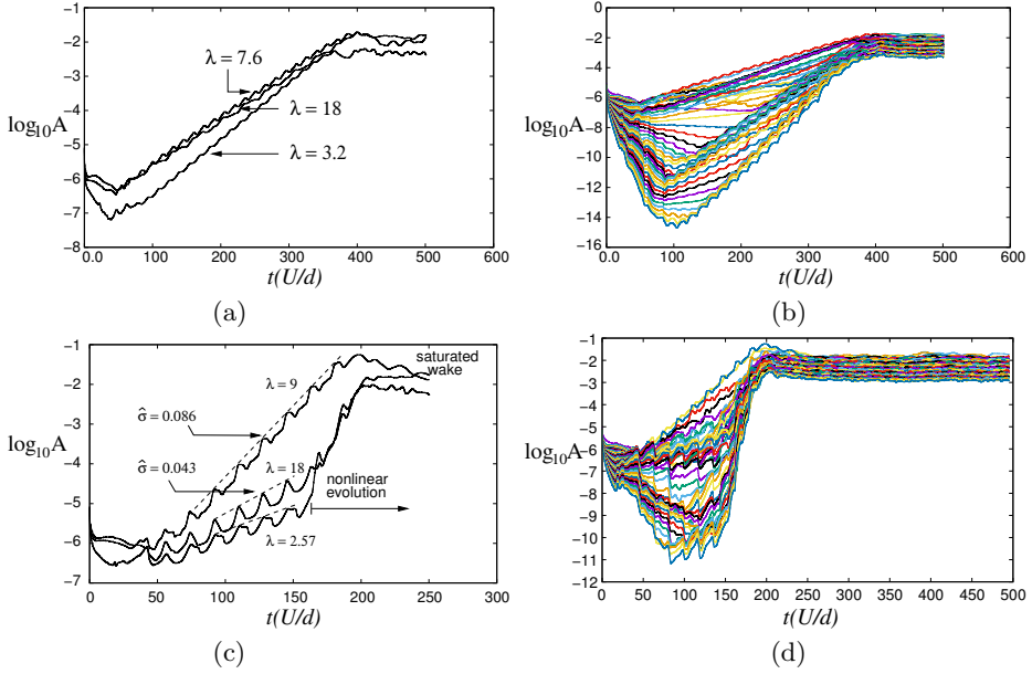
Figure 20: Evolution of the amplitude of spanwise Fourier modes at different Reynolds numbers. Top row: Re = 100 ; bottom row: Re = 160 . The subfigures on the left show the evolution of the three dominant wavelengths as predicted by Floquet analysis, and those on the right show the evolution of the amplitudes corresponding to the first 48 modes. The simulations are started impulsively, with a low level white noise to accelerate the development of the three-dimensionality. Measured slopes of the evolution curves in the linear regime give estimated growth rates ( \hat{\sigma} ) in agreement with growth rate predictions from Floquet analysis given in figure 11.
