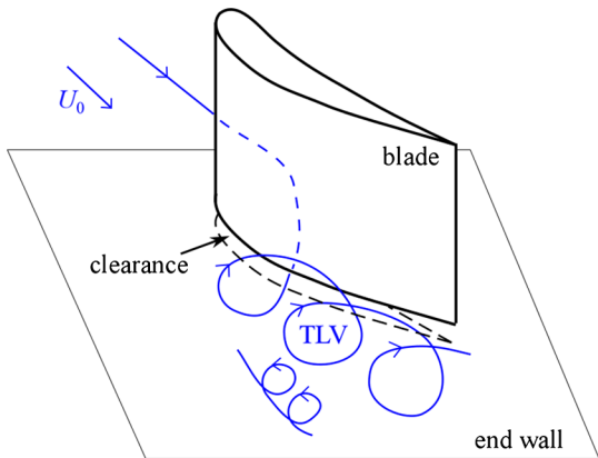
Fig. 1 Sketch of a tip-clearance flow.
