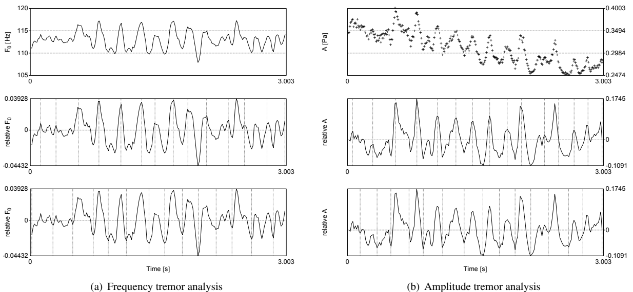
Fig. 1. Steps of tremor analysis: The upper sub-figures show the F_0 and the amplitude ( A ) contour, the middle sub-figures depict the normalized and de-declined contours with time marks at the tremor maxima. The lower sub-figures show time marks for the tremor minima. Fig. (a) shows the frequency and Fig. (b) the amplitude tremor analysis of a 3 seconds lasting quasi-stationary part of the sustained vowel /a/ from a male speaker (id 19) of the AHN corpus. At the recording time he was 74.24 years old, PD patient, and off medication. FTrF=4.75Hz, FTrI=2.019%, FTrP=1.668, ATrF=4.64Hz, ATrI=6.462%, ATrP=5.316.
