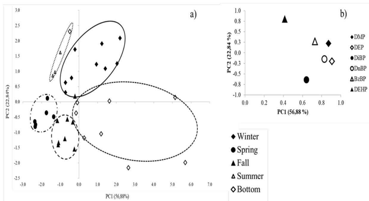
Figure 6. Principal components analysis (PCA) for PAEs in the study area was applied to reduce the multidimensional nature of the dataset and to evaluate the interrelationships among the PAEs, sites and sampling periods. The PCA statistics were performed using the statistical package XLSTAT 2010.2 (Addinsoft). In (a) the sample scores, whereas in (b) the variable loadings of the PCA. The variance accounted for by each principal component is shown in parentheses after the axis label.
