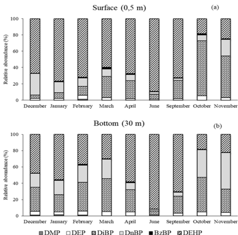
249 Figure 5. Relative abundance of PAEs in surface (0.5 m; a) and bottom (30 m; b) seawater samples collected 250 at SUNMEX station in Marseille Bay from December 2013 to November 2014. 251
