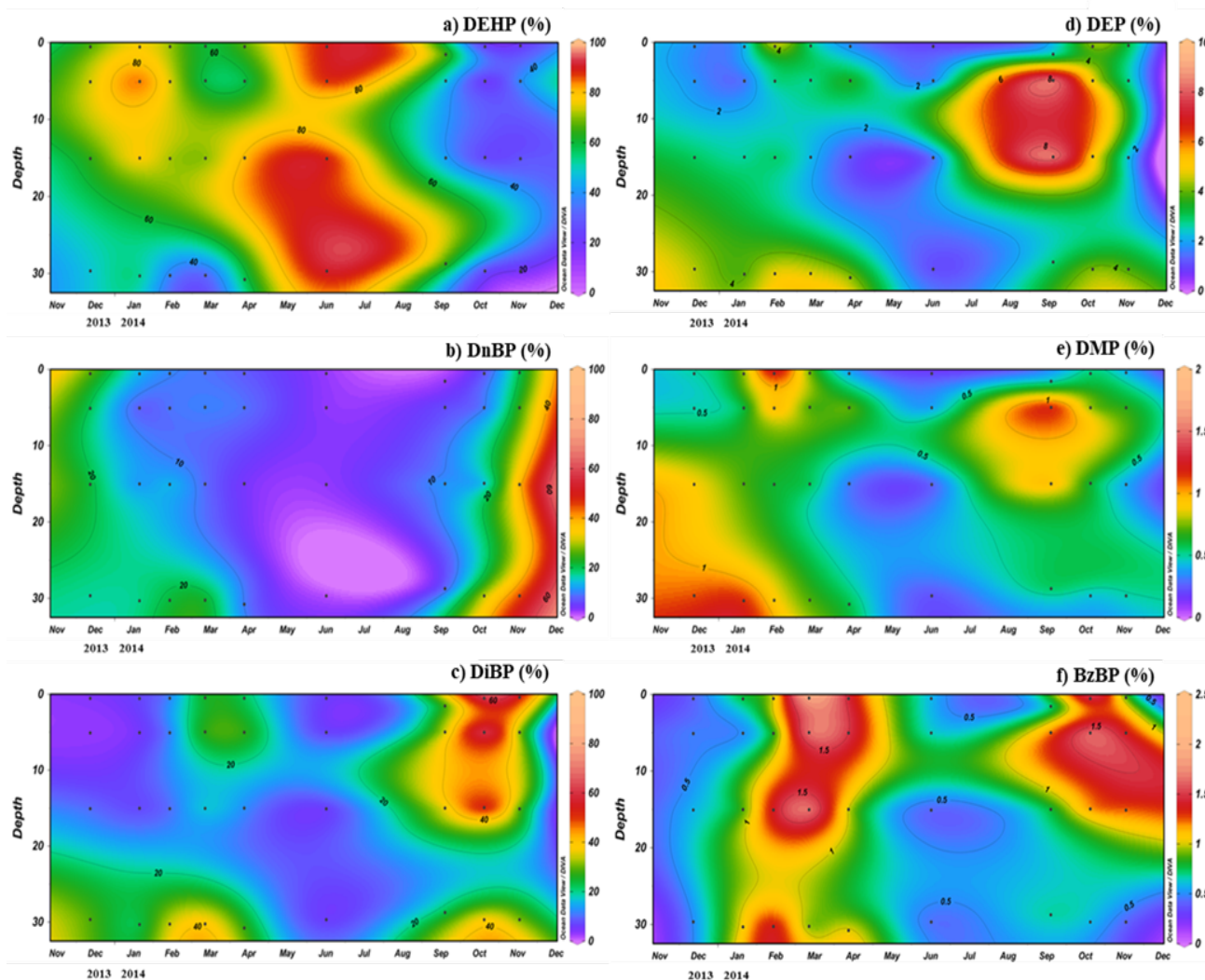
Figure 4. Relative abundances for DEHP (a), DnBP (b), DiBP (c), DEP (d), DMP (e) and BzBP (f) at SUNMEX station in Marseille Bay from December 2013 to November 2014.
