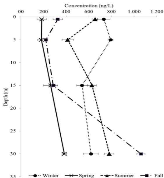
314 315 Figure 7. \Sigma PAEs vertical profile at Bay of Marseille in 4 seasons (average values) of 2014. 316
