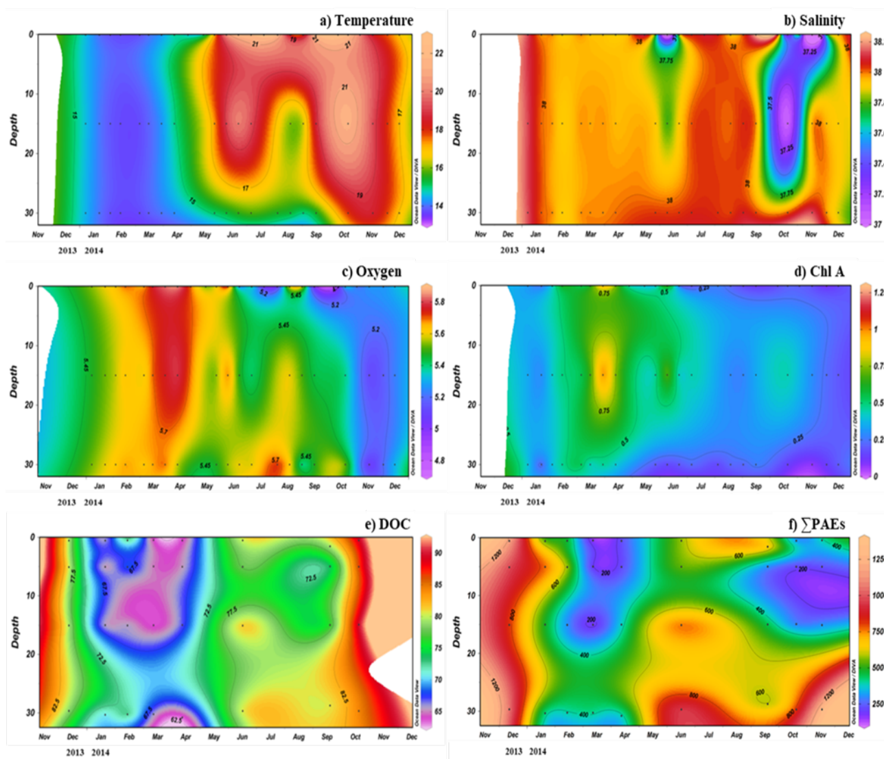
200 Figure 3. a) Temperature ( ^{\circ}\text{C} ), b) salinity (PSU), c) oxygen ( \text{ml L}^{-1} ), d) chlorophyll A ( \mu\text{g L}^{-1} ), e) DOC ( \mu\text{M} ) 201 and f) \Sigma\text{PAEs} ( \text{ng L}^{-1} ) time-series at SUNMEX station (Bay of Marseille) from December 2013 to 202 November 2014. Samples were collected at 1.5, 5, 15 and 30 m.
