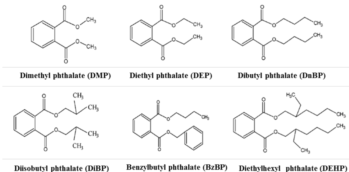
Figure 2. Chemical structure of the 6 detected PAEs. Dimethyl phthalate (DMP; MW = 194.18), Diethyl phthalate (DEP; MW = 222.24), Dibutyl phthalate (DnBP; MW = 278.34), Diisobutyl phthalate (DiBP; MW = 278.34), Benzylbutyl phthalate (BzBP; MW = 312.36) and Diethylhexyl phthalate (DEHP; MW = 390.56). Figure adapted from Xie et al. 7
