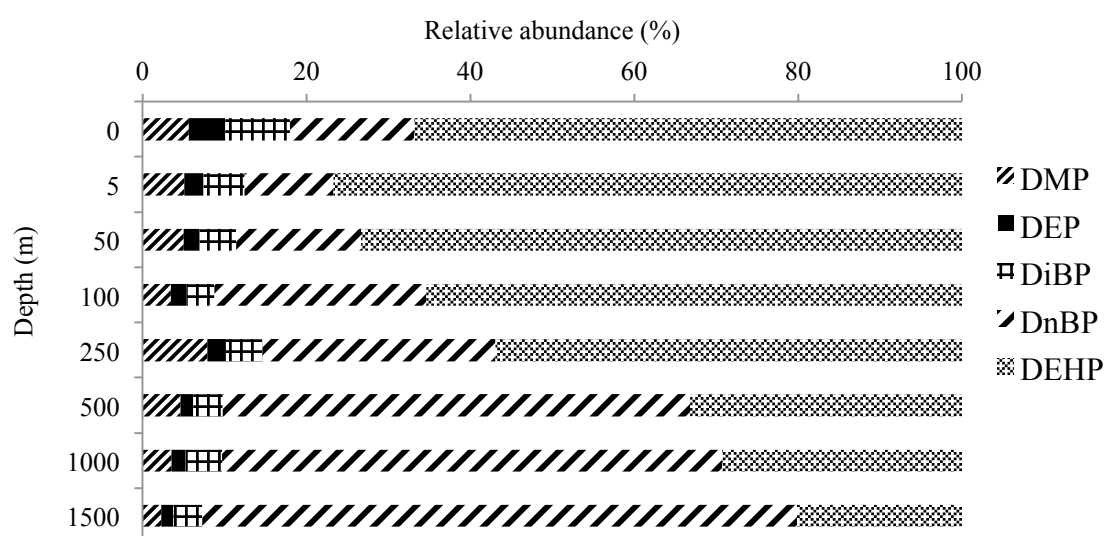
Figure 5. PAE relative abundances (%) detected in offshore Antares station-samples collected at the surface and at depths of 5, 50, 100, 250, 500, 1000 and 1500 m in March 2015.
