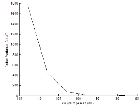
Fig. 13 Phase noise variance vs. signal power at VNA input at d = 1 m and f_e = 20 GHz
