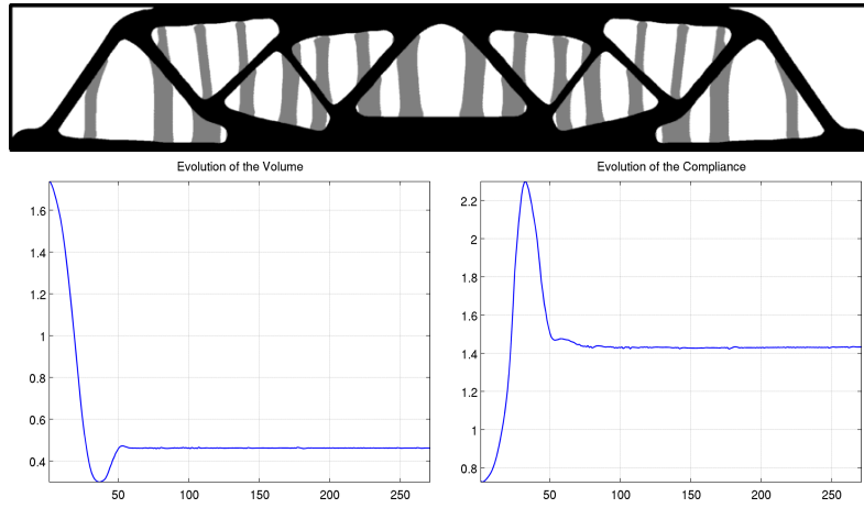
Figure 4: Optimal supports and convergence curves for Test Case 1 with a volume constraint and an augmented Lagrangian algorithm. Fixed shape and initialization given in Figure 2
