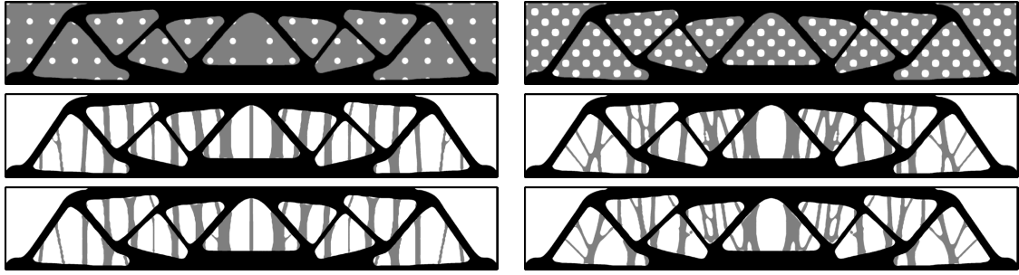
Figure 21: Test Case 12: Optimization of the supports for a MBB beam for 10 (middle line) and 50 slices (bottom line), for different initial conditions at fixed volume (top line). The optimized designs on the left, giving rise to vertical bar structures, have a lower value of the cost function.
