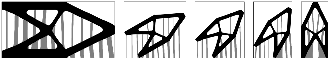
Figure 19: Optimal supports for different orientations 0^\circ , 30^\circ , 45^\circ , 60^\circ and 90^\circ of the fixed shape. The support has fixed volume in all computations. The cantilever shapes have the same size, but the pictures are rescaled to have a fixed height.
