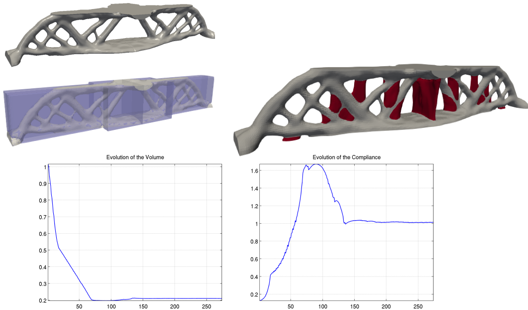
Figure 11: Test Case 6 (3D beam): fixed shape and initial (left) and the optimized support (right) together with the convergence curves.
