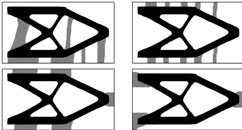
Figure 14: Test Case 8: Optimal supports for thermal evacuation with different boundary conditions: bottom, top-bottom, top-bottom-right and left-right.
