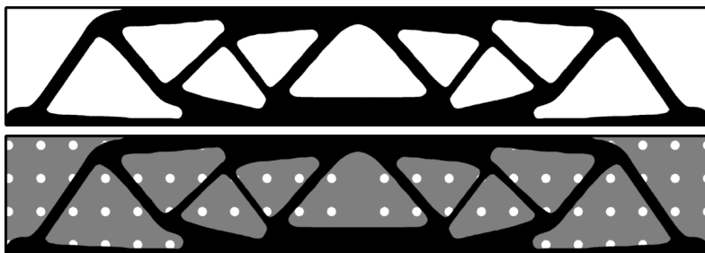
Figure 2: The fixed shape and the initialization used for Test Case 1 (MBB beam).
