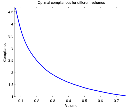
Figure 5: Optimal compliance of the supported structure as a function of the support volume constraint for Test Case 1.
