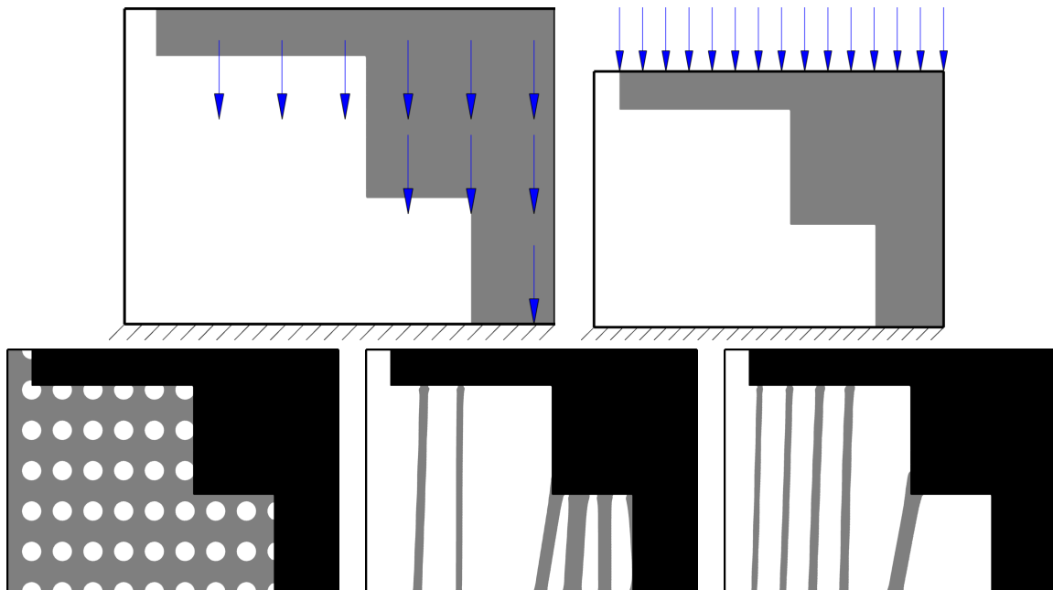
Figure 9: (top row) Loadings considered for the Test Case 4 inspired from [30]. On the left, bulk loads as proposed in the present work, while on the right, for the sake of comparison, surface loads as proposed in [30]. (bottom row): initial support (left), result for the model proposed in this article using bulk loads (center), result for the model using surface loads on the upper boundary as in [30] (right).
