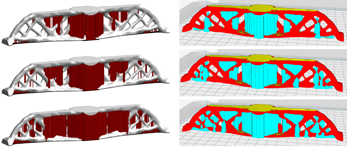
Figure 12: (left) Vertical supports generated under the overhang regions for the fixed beam shape shown in Figure 11 for limiting angle \alpha_0 \in \{21.5^\circ, 30^\circ, 45^\circ\} . (right) Supports generated by the freeware software Ultimaker Cura for the same angles.
