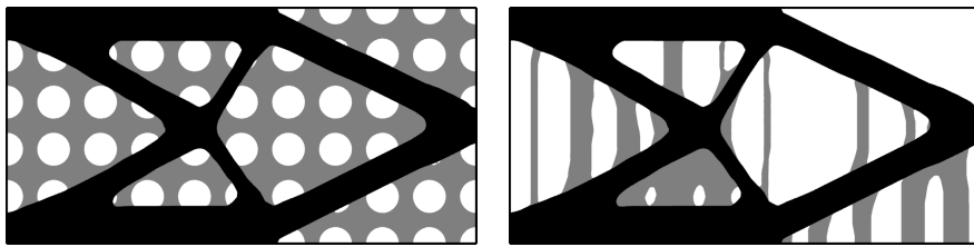
Figure 13: Test Case 7: initial and optimal supports for thermal evacuation.
