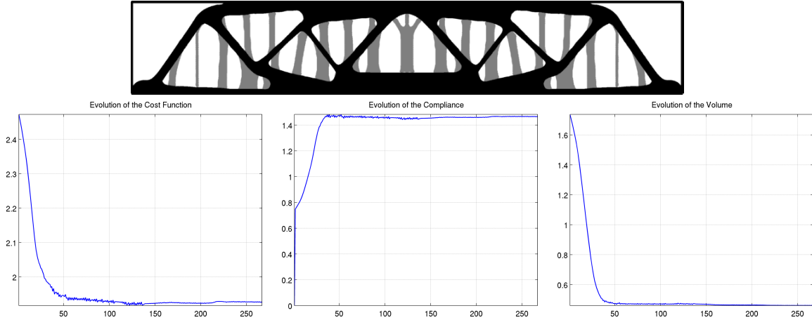
Figure 3: Optimal supports and convergence curves for Test Case 1 with a fixed Lagrange multiplier \ell = 1 . Fixed shape and initialization given in Figure 2
