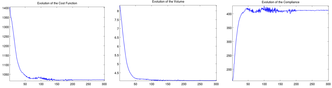
Figure 7: Convergence history of the cost function, the volume and the compliance for Test Case 2 (M-shape).
