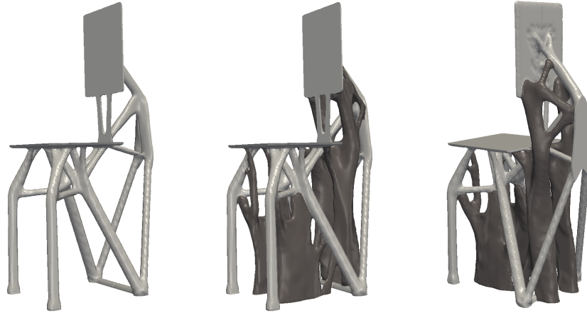
Figure 10: Test Case 5 (3D chair): fixed shape (left) and two views of the optimal supports.
