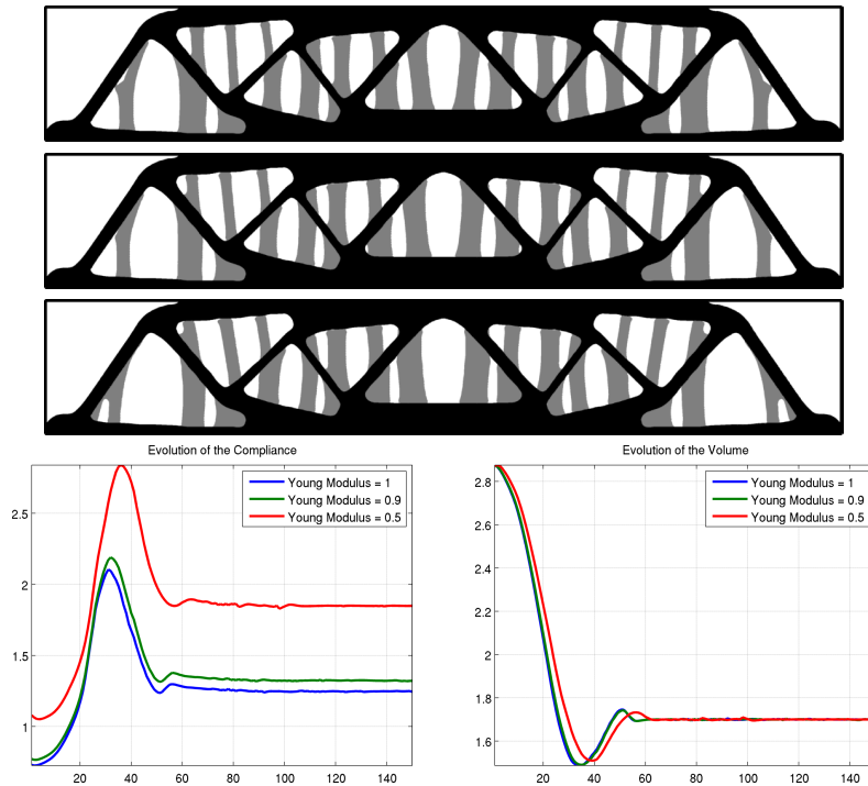
Figure 8: Test Case 3: optimal supports and convergence histories obtained when varying the Young modulus of the support. The Young modulus of the support is equal to 1, 0.9 and 0.5 (from top to bottom), while for the shape it is kept at 1.
