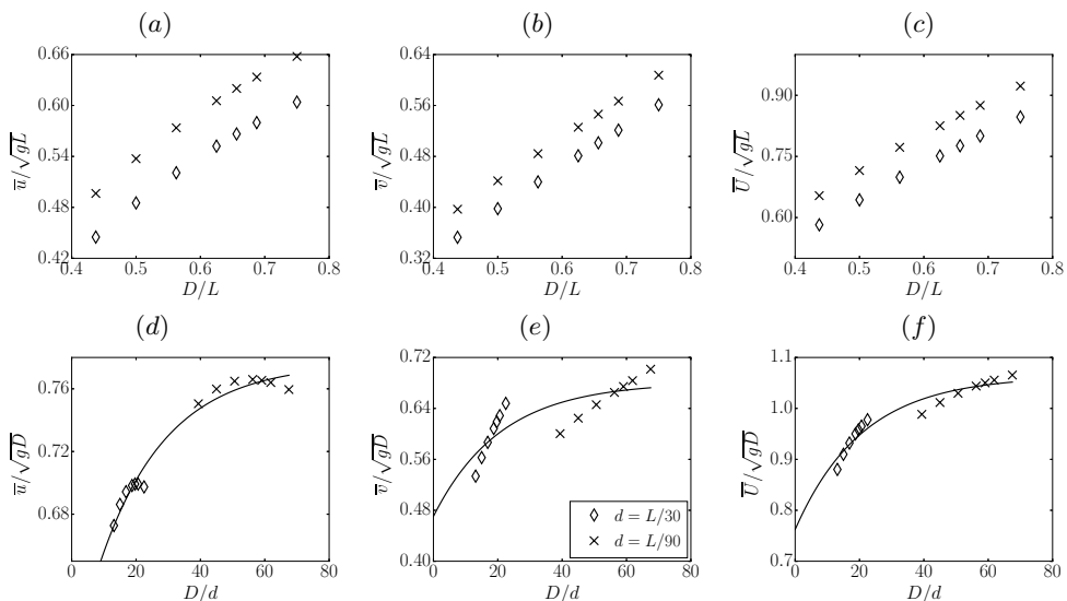
Figure 19: 2D continuum simulation (a,d) horizontal velocity, (b,e) vertical velocity, and (c,f) norm of the velocity normalised in (a,b,c) by \sqrt{gL} versus D/L and normalised in (d,e,f) by \sqrt{gD} versus D/d for two particles diameters. The full lines in (d,e,f) represent equation A 6 with the fitting parameters \beta = 0.05 , \xi_u = 0.78 , \alpha_u = 0.25 , \xi_v = 0.68 , \alpha_v = 0.31 , \xi_U = 1.06 and \alpha_U = 0.28 obtained using the least squares method.
