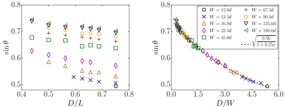
Figure 9: Continuum simulation results: angle of inclination \theta of the central streamline at the orifice relative to vertical for various W (a) versus D/L , (b) versus D/W . The dashed line represents equation 3.10 with \gamma_1 = 0.56 and \gamma_2 = 0.25 .
