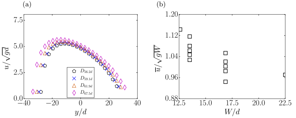
Figure 20: Pseudo-3D continuum simulation. (a) Horizontal velocity normalized by \sqrt{gd} versus y/d at the outlet for different D and W = 13.5d (b) mean horizontal velocity normalised by \sqrt{gW} for D/W > 3 .
