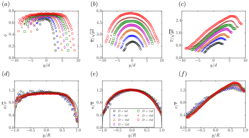
Figure 15: (Color online)(a-f) Flow of particles of diameter of d = 2 mm for different outlet diameters. Vertical profiles of (a) the volume fraction, \phi , (b) the horizontal velocity, u , and (c) the vertical velocity, v , versus the vertical position, y . Vertical profiles of (d) the volume fraction normalised by the mean volume fraction, \bar{\phi} , (e) the horizontal velocity made dimensionless by the mean horizontal velocity, \bar{u} , and (f) the vertical velocity made dimensionless by the mean vertical velocity, \bar{v} , versus the position normalised by the outlet radius ( R = D/2 ). The full lines represent in (d) Eq. A 3 with \nu_\phi = 0.21 and in (e) Eq. A 4 with \nu_v = 0.38 respectively.
