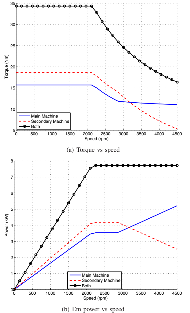
Fig. 6. Torque and power with CPR-MTPA strategy
