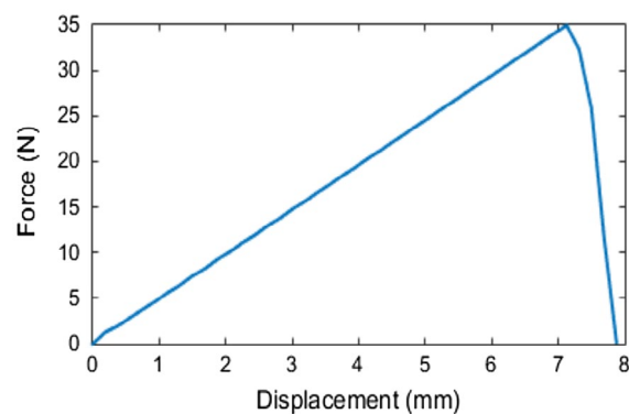
Figure 2. Force-displacement curve from uniaxial tensile test simulation along longitudinal fibres.
