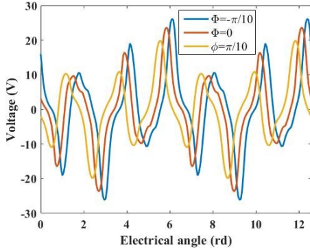
Fig. 8. Voltage waveform for three values of phase shift \phi and a current density of 20\text{A}/\text{mm}^2 obtained by FE simulation.
