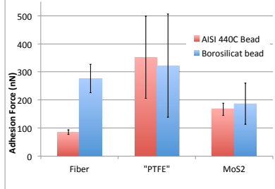
1.1.1 Figure 6 – AFM mean results of pull-off force for PGM-HT.
