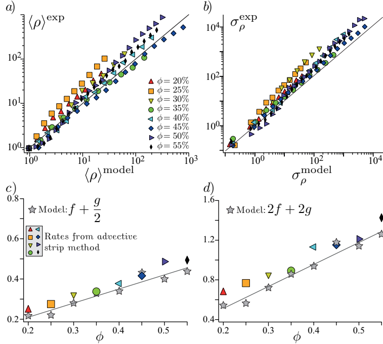
FIGURE 12. Comparison between the experimental stretching (extracted from figure 8) and the multiplicative stretching model. (a-b) Mean elongation \langle \rho \rangle and standard deviation \sigma_\rho . The values from the advective strip method are plotted versus those predicted by the multiplicative stretching model. (c) Comparison between the exponential rates of the mean elongation \kappa_\rho obtained from the advective strip method (see figure 8a) and the model prediction f + g/2 (5.12). (d) Comparison between the exponential rates of the variance of the elongation 2\kappa_{\sigma_\rho} (see figure 8b) and the model prediction 2(f + g) (5.13).
