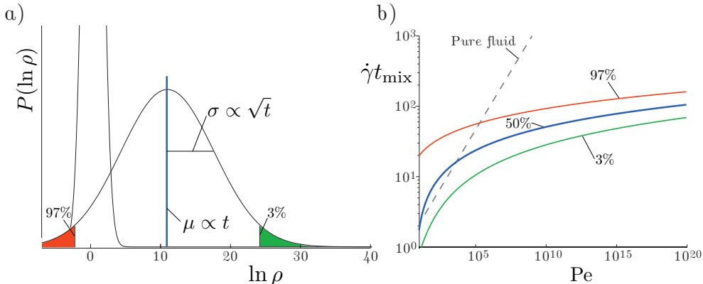
FIGURE 15. a) Evolution of the distribution P(\ln \rho) of the logarithm of the material line elongations in a particulate suspension. The mean of the distribution \mu \sim t and its standard deviation \sigma \sim \sqrt{t} . b) Dimensionless mixing times \dot{\gamma} t_{\text{mix}} in a suspension ( \phi = 35\% ) as a function of Pe . The median (blue line), the most stretched t_{\text{mix}}^{3\%} (green line), and the less stretched t_{\text{mix}}^{97\%} (red line) dimensionless mixing times can be compared to the dimensionless mixing time \sim Pe^{1/3} expected in a pure fluid (dashed line).
