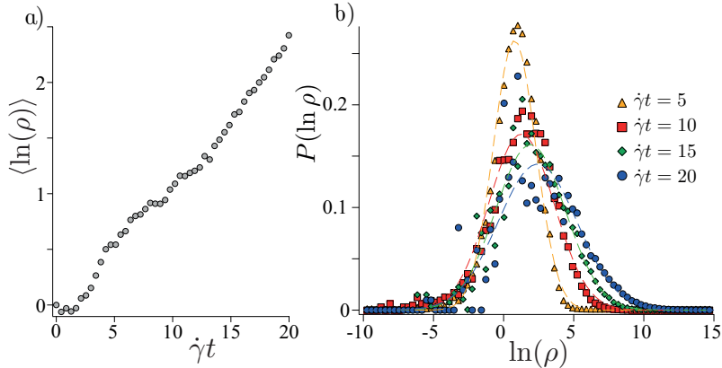
FIGURE 13. a) Mean logarithm of the material line elongations, \langle \ln \rho \rangle versus \dot{\gamma}t for a suspension of volume fraction \phi = 35\% . b) PDF of the logarithm of the material line elongations P(\ln \rho) at successive times.
