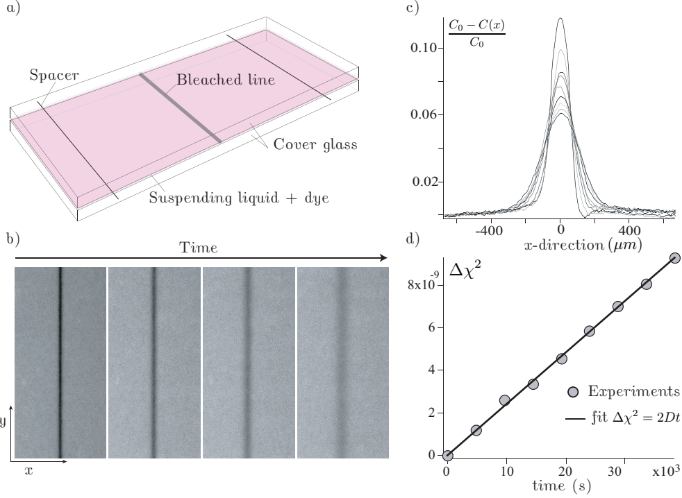
FIGURE 4. a) Schematics of the set-up used to measure the molecular diffusivity D of the dye (rhodamine 6G), in the suspending liquid (TritonX+ZnCl 2 +H 2 O). b) Diffusive thickening of the bleached line at t = 0, 4800, 21600 and 64800 s (the image width is 5 mm). c) Concentration profiles at successive times ( 0 \text{ s} < t < 64800 \text{ s} ). d) Increase of the spatial variance of the concentration \chi^2(t) - \chi^2(0) versus time. Its fit to 2Dt yields D = 1.44 \pm 0.2 \times 10^{-13} \text{ m}^2 \text{ s}^{-1} .
