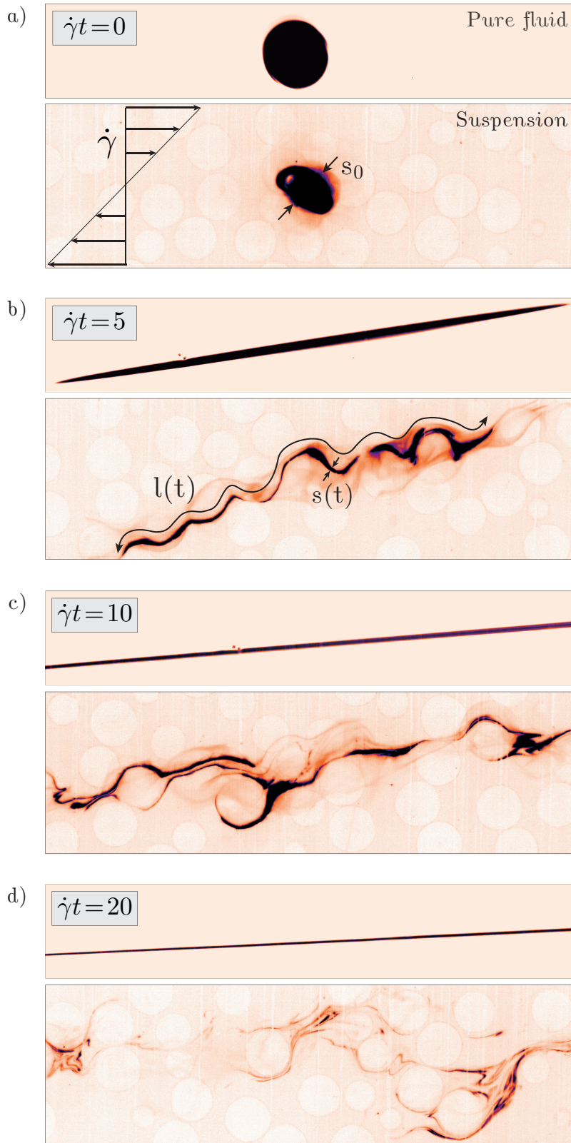
FIGURE 5. Comparison of the stretching processes of a blob of dye sheared at high Péclet ( \sim 10^6 ) and low Reynolds numbers ( \sim 10^{-4} ), in a pure fluid (top), and in a particulate suspension with volume fraction \phi = 35\% (bottom). The dye appears as dark, and the beads appear as bright, see also Movie 2.
