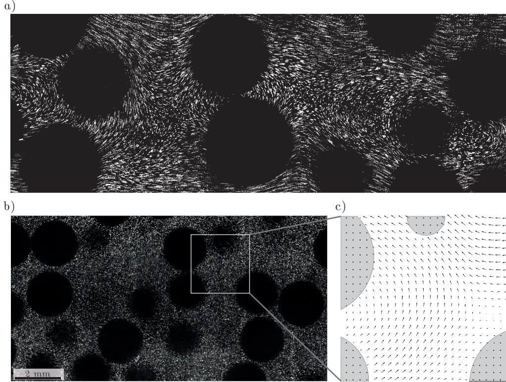
FIGURE 3. a) Flow streamlines in the bulk of a suspension. b) Slice of a sheared suspension illuminated by a laser sheet. The small fluorescent tracers seeding the suspending fluid appear as bright whereas the particle intersections with the laser sheet appear as dark, see also Movie 1. c) Magnified view of the suspending liquid velocity field obtained from the PIV (the velocity is not computed in the particles).
