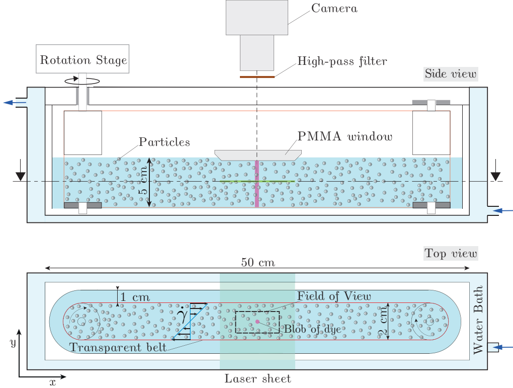
FIGURE 2. Schematics of the set-up.
