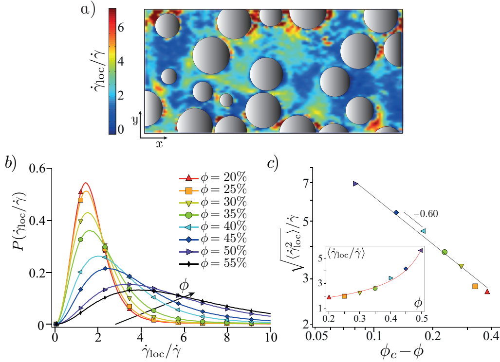
FIGURE 10. a) Typical local shear rate map for a suspension with volume fraction \phi = 35\% . b) Experimental distributions of normalized local shear rate P(\dot{\gamma}_{\text{loc}}/\dot{\gamma}) for different volume fractions (the solid line is not a fit but the experimental data, sparse markers are used for sake of clarity). c) \sqrt{\langle \dot{\gamma}_{\text{loc}}^2 \rangle}/\dot{\gamma} versus \phi_c - \phi . The best fit \sqrt{\langle \dot{\gamma}_{\text{loc}}^2 \rangle}/\dot{\gamma} \sim (\phi_c - \phi)^{-\beta} , with \phi_c = 0.58 , yields \beta = 0.601 (see text). Inset: mean normalized local shear rate \langle \dot{\gamma}_{\text{loc}}/\dot{\gamma} \rangle versus \phi . The line is the best fit by A/(\phi_c - \phi)^\delta .
