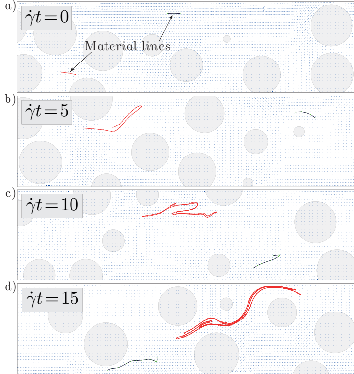
FIGURE 6. Example of stretching for two material lines numerically advected using the experimental fluid velocity field, see also Movie 3.
