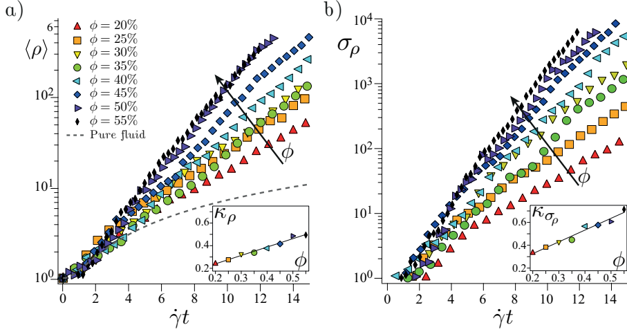
FIGURE 8. Mean elongation \langle \rho \rangle (a) and standard deviation \sigma_\rho (b) versus strain for increasing volume fractions ranging from 20 to 55%. Insets: growth rate \kappa of the exponential fit e^{\kappa \dot{\gamma} t} to the main curves, as a function of \phi . The lines show \kappa_\rho = 0.09 + 0.74 \phi (a), and \kappa_{\sigma_\rho} = 0.12 + 1.03 \phi (b).
