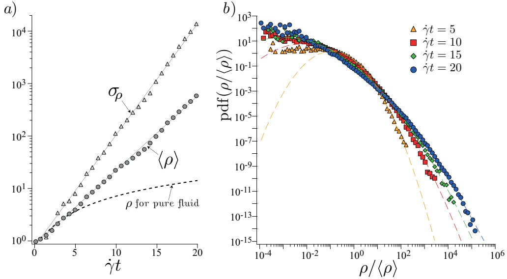
FIGURE 7. Stretching laws measured for a suspension with volume fraction \phi = 35\% . a) Mean value \langle \rho \rangle and standard deviation \sigma_\rho = \sqrt{\langle \rho^2 \rangle - \langle \rho \rangle^2} of the distribution of elongations versus macroscopic strain in a semilogarithmic representation. The dashed line corresponds to the mean elongation in a pure fluid \rho_{\text{lin}}(t) = \sqrt{1 + \dot{\gamma}^2 t^2}/2 . b) Distribution of the normalized elongations \rho/\langle \rho \rangle at different strains. The dashed curves are log-normal distributions built from the mean value \langle \rho \rangle and standard deviation \sigma_\rho of the experimental elongation distributions.
