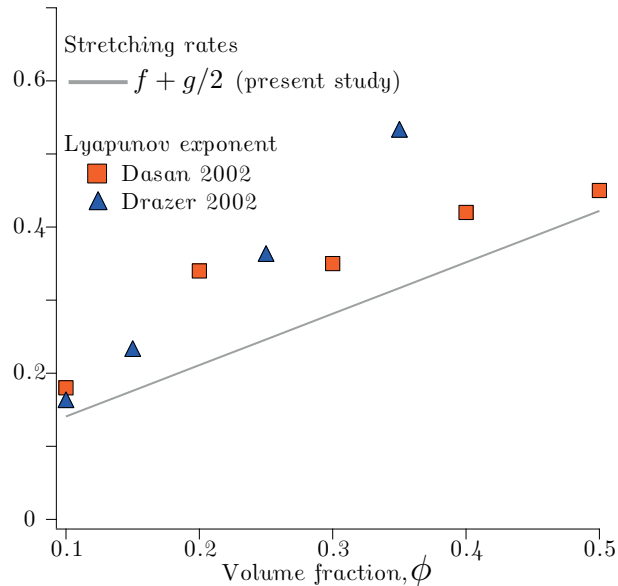
FIGURE 14. Comparison between the stretching rates obtained in the present study and the largest Lyapunov exponent obtained from 3D Stokesian dynamics simulations (Dasan 2002, Drazer 2002).
