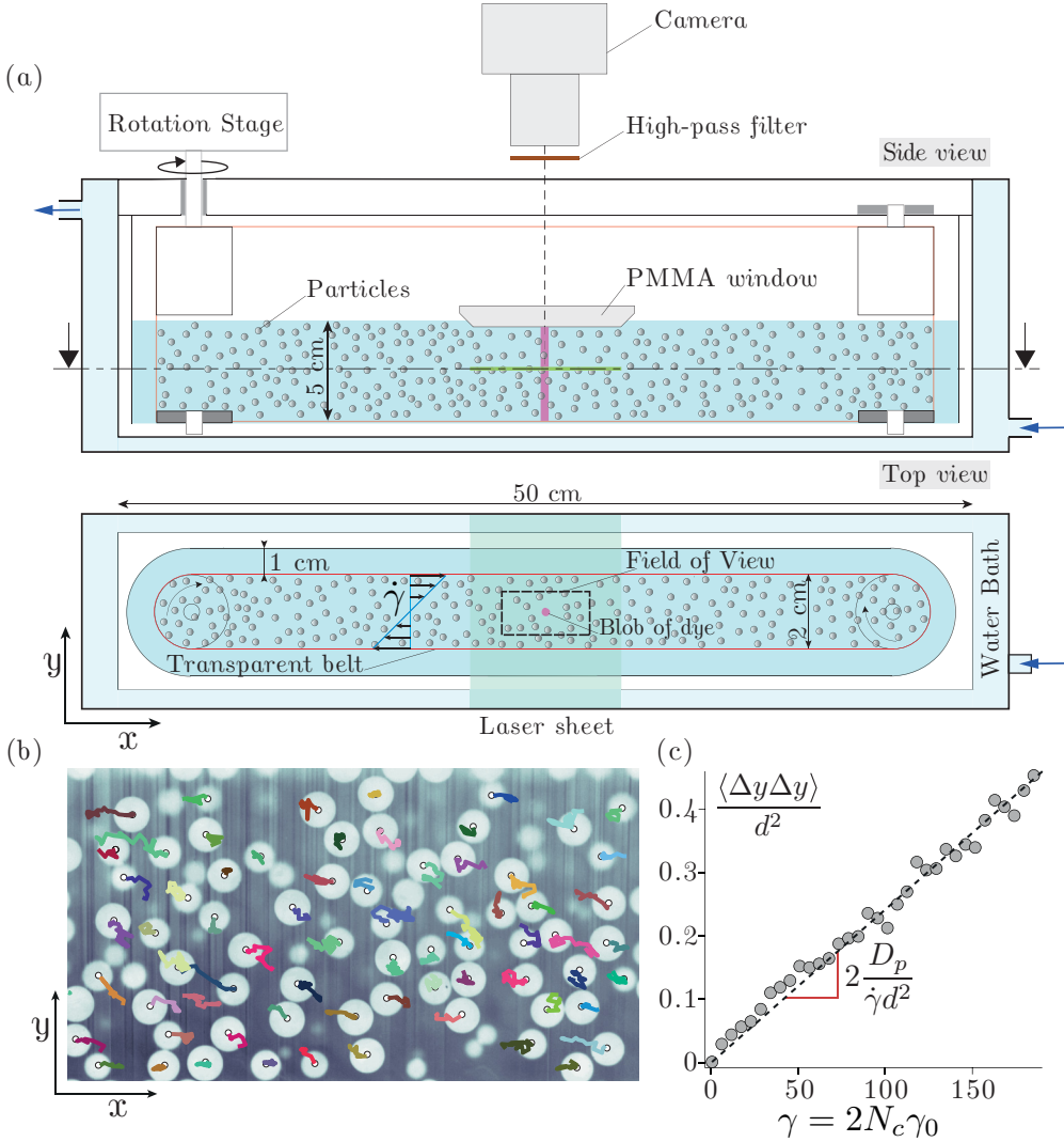
FIG. 1. (a) Schematic of the setup, top and side views. (b) Image of the suspension seen from the top (particles appear as white discs) and stroboscopic particle trajectories for cycles of shear of strain amplitude \gamma_0 = 2.8 . (c) Corresponding particle mean square displacement versus total accumulated strain \gamma = 2N_c \gamma_0 .
