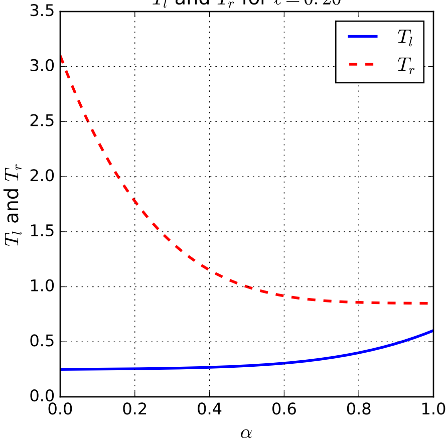
T_l and T_r for \ell = 0.20
