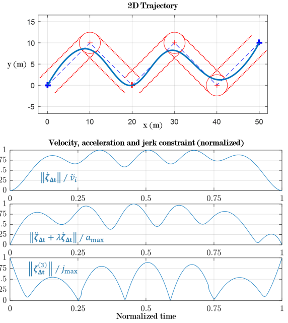
Fig. 3. Example of minimum jerk trajectory
