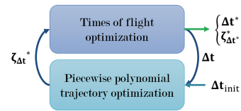
Fig. 2. Bilevel optimization strategy for generating the trajectory
