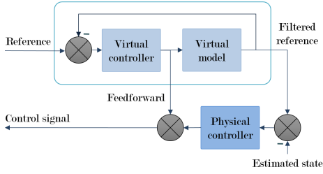
Fig. 6. Architecture of the heading controller
