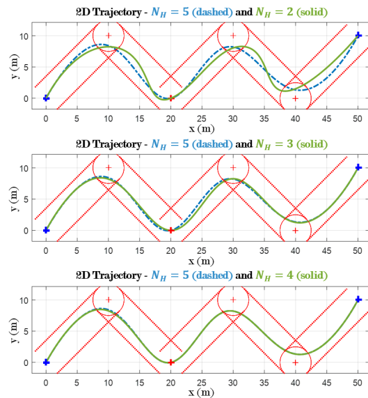
Fig. 5. Optimality loss induced by the receding horizon strategy when decreasing N_H
