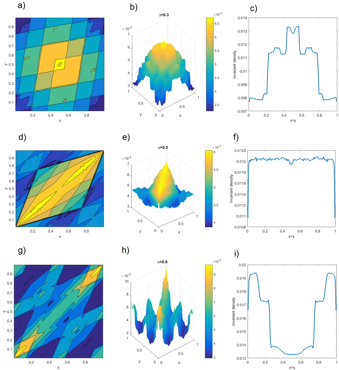
FIGURE 1. Invariant density for the map 2.2 with n = 2 for \gamma = 0.3 (a,b,c), \gamma = 0.5 (d,e,f), \gamma = 0.6 (g,h,i). The plots show the density in colorscale (a,d,g) with a view from the top and (b,e,h) for a three dimensional view. The plots (c,f,i) show the behavior of the map on the diagonal. The figure is obtained by averaging the density over 300 realizations each consisting of 10^7 iterations of the trajectory.
