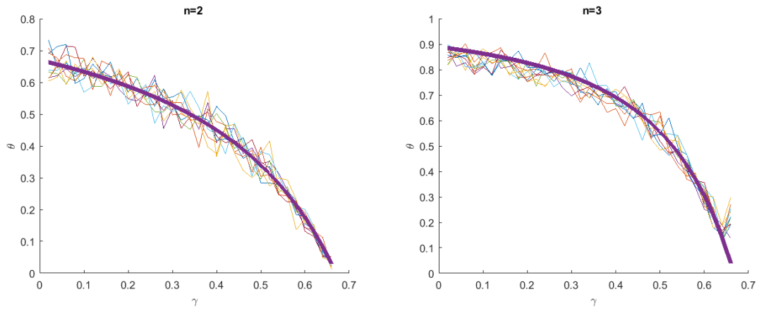
FIGURE 6. Extremal index \theta of the Generalized Pareto distribution as a function of the coupling parameter \gamma . Thin lines indicate estimates for 10 different realization of the maps 3x \text{-mod } 1 . Bold magenta lines indicate the expected theoretical values. Left: n = 2 , Right: n = 3 .
