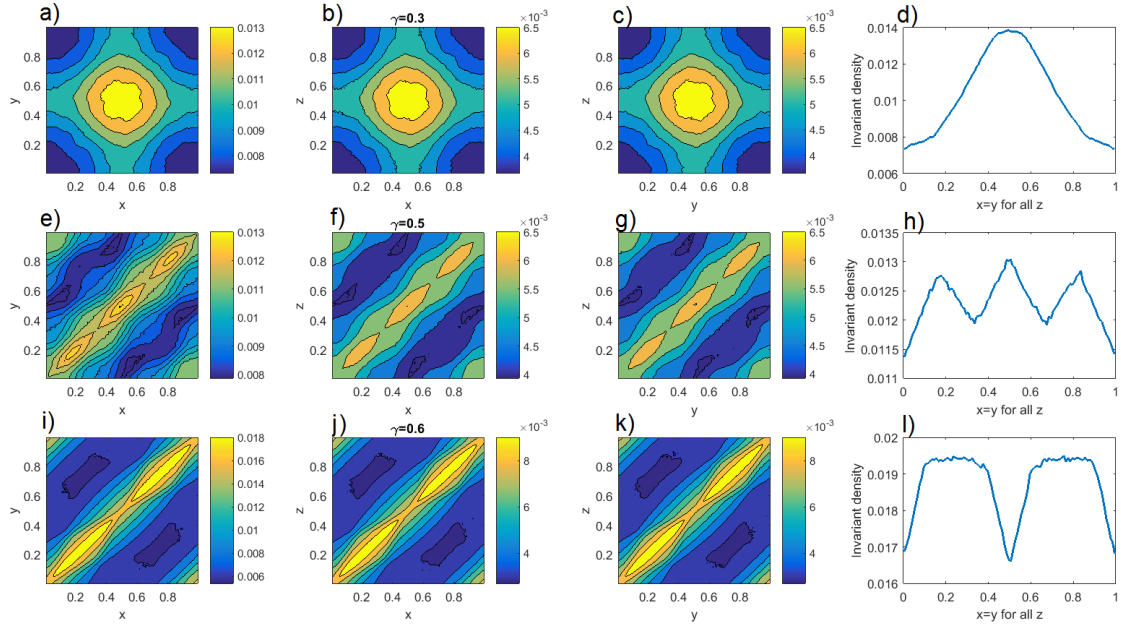
FIGURE 2. Invariant density for the map 2.2 with n = 3 for \gamma = 0.3 (a,b,c,d), \gamma = 0.5 (e,f,g,h), \gamma = 0.6 (i,j,k,l). The plots show the density in colorscale (a-c,e-g,i-k). The plots (d,h,l) show the behavior of the map on the diagonal x = y . The figure is obtained by averaging the density over 300 realizations each consisting of 10^6 iterations of the trajectory.
